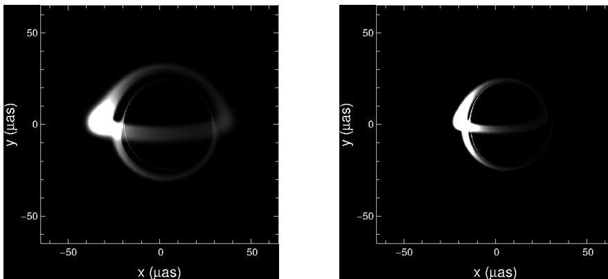
Fig. 1 The images of an optically thin ion torus around a moderately (left) and fast (right) spinning Kerr black hole as observed by an observer on Earth (see [24] for details).
