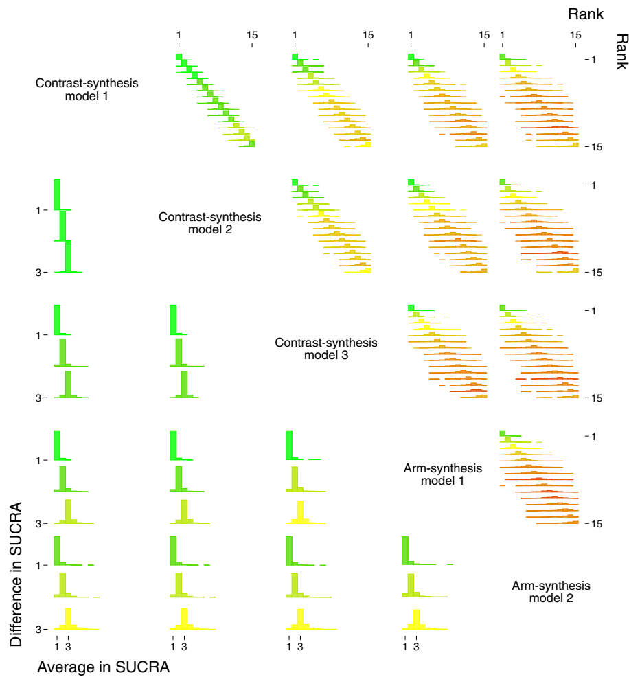
Fig. 4 Comparison of rankings obtained from the five methods used to synthesise evidence from network meta-analyses. Note that the data pictured have been simulated for illustrative purposes
