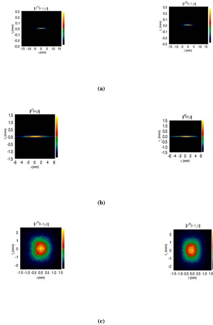
Fig 2 The experimentally reconstructed projection of the spatial coherence functions nm along (Left) x -direction J^{(1)}(x, s_x, \theta) and (right) y -direction J^{(2)}(y, s_y, \theta) of two-dimensional field (a) at the output face of the LED source peaked with a wavelength of 665 \pm 10 nm and bandpass of 10, (b) at the output face of the fibre collimating lens of the filtered multi-mode fibre-coupled white (white) light source with centre wavelength 521nm and (c) collimated
