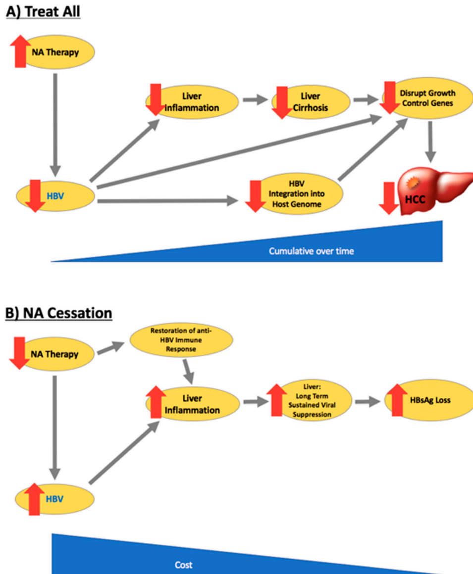
Figure 1. Benefits of “treat all” and nucleos(t)ide analogue (NA) cessation: HBsAg loss rates and hepatocellular carcinoma (HCC)/cirrhosis risk. (A) “Treat all” reduces HBV viraemia, hepatic inflammation, and thus cirrhosis and HCC risk; (B) “NA cessation” causes an initial HBV viral relapse with subsequent increase in rates of HBsAg loss.
