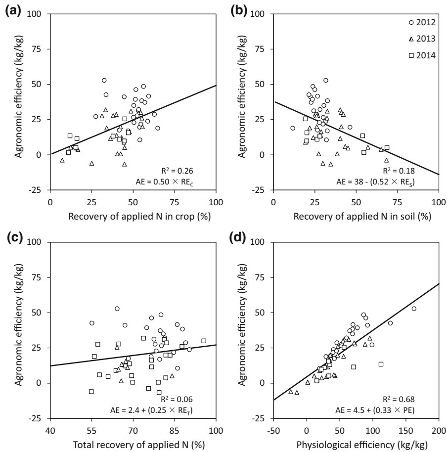
Fig. 4 Relationship between agronomic efficiency of N fertiliser application (kg/kg) and recovery of applied N (%) in crop (a), soil (b), total (c), physiological efficiency (d) of N fertiliser application (kg/kg). Solid lines represent the result of linear regression between the two factors
