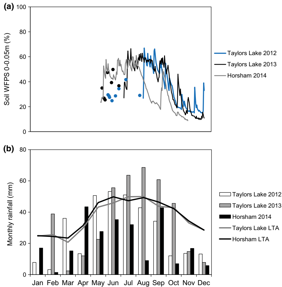
Fig. 2 Daily soil WFPS (0–0.05 m) during the growing season (a) and monthly rainfall totals during the experimental period and long-term average (LTA) at Taylors Lake and Horsham (b). Rainfall data for September 2014 includes 31 mm of irrigation. Soil WFPS prior to 14-August 2012 and 6-July 2013 based on soil cores, thereafter measured using continuous logging soil moisture probes
