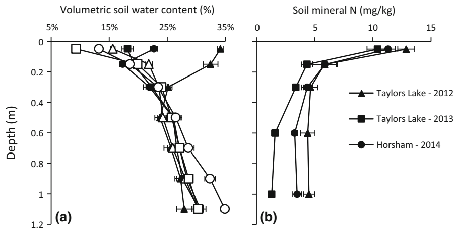
Fig. 1 Volumetric soil water content (%) immediately prior to sowing (closed captions) and averaged across treatments at harvest (open captions) (a), soil mineral N content (mg/kg) at sowing (b) to a depth of 1.2 m at Taylors Lake in 2012 and 2013 and Horsham in 2014. Error bars represent standard error of the mean ( n = 5 at sowing, n = 25 at harvest)
