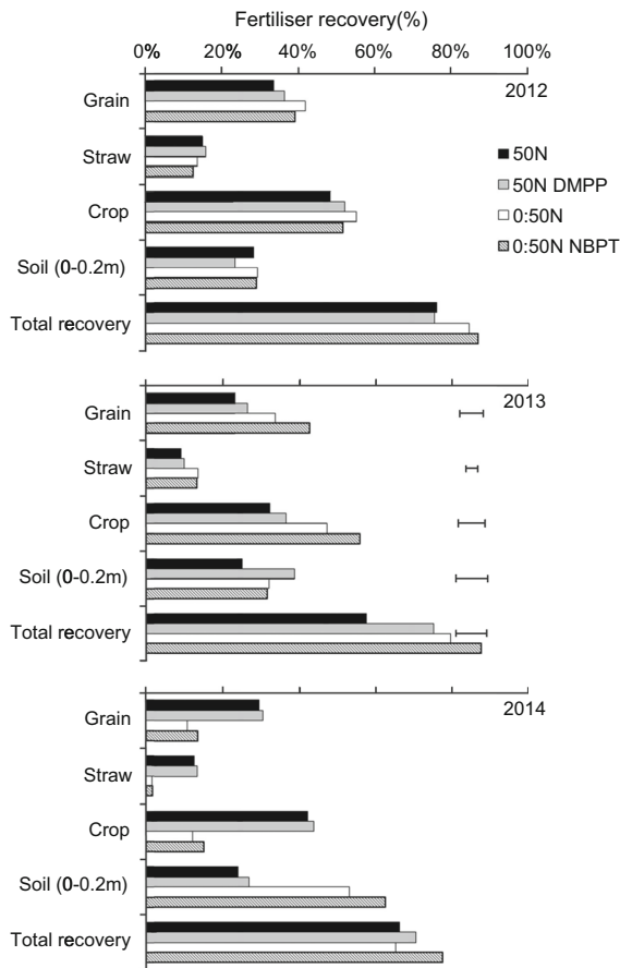
Fig. 3 Recovery (%) of applied N at harvest in grain, straw, aboveground biomass (crop), soil (0–0.2 m) and in total (sum of crop and soil) in relation to N fertiliser treatment at Taylors Lake in 2012 and 2013 and Horsham in 2014. Error bars represent least significant ( P < 0.05 ) differences for each variable when comparing treatments within a given year
