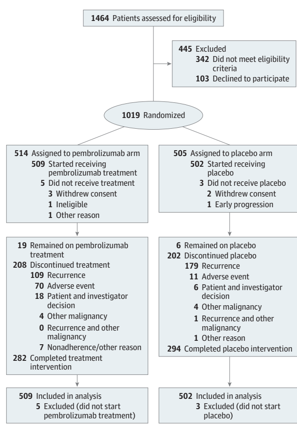
Figure 1. CONSORT Diagram
