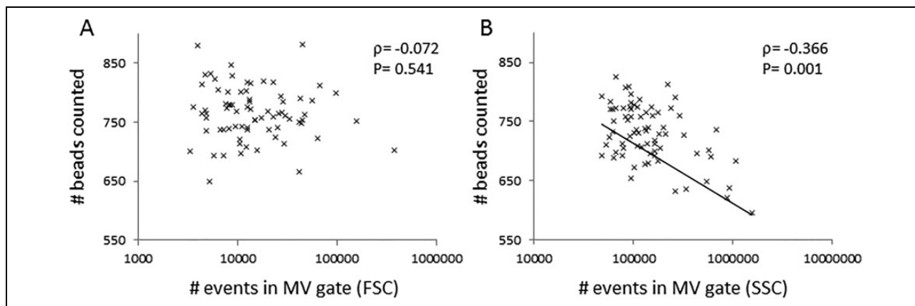
Figure 3. Correlation between the number of beads counted and the number of MV events detected by SSC. Scatterplots show relationship between the number of beads counted and the number of MV events detected in the MV gate when using (a) FSC or (b) SSC as the main detection parameter.
