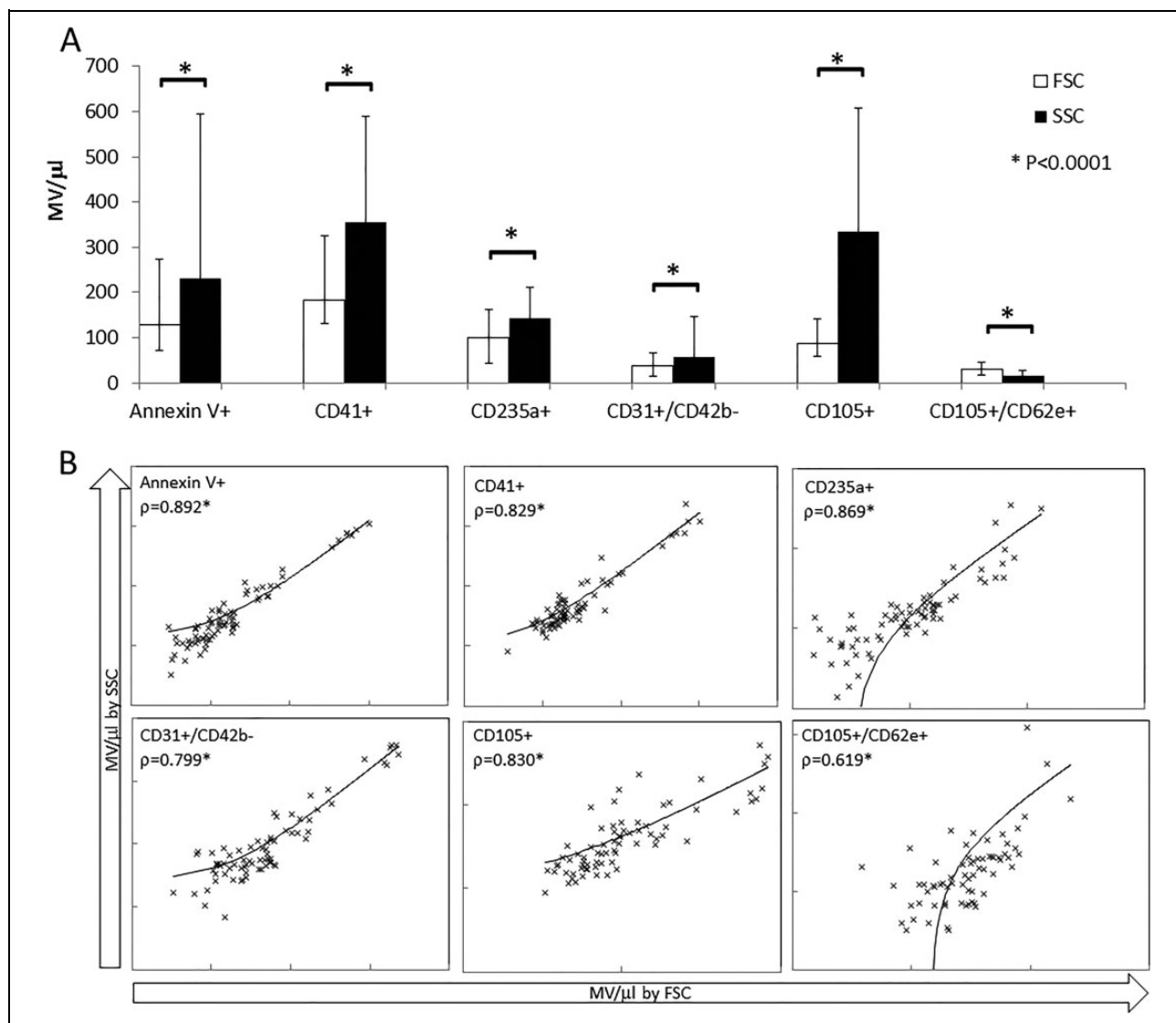
Figure 4. Results of MV subsets calculated from data using FSC or SSC as the main detection parameter. (a) Bar graph illustrating differences in concentrations of MV subsets when calculated from data obtained using FSC versus SSC as the main detection parameter. Bars represent median and interquartile ranges. (b) Correlation of individual MV subset concentrations when calculated from data obtained using FSC versus SSC as the main detection parameter. Scatter graphs are presented on log scales. * p < 0.0001 . MV: microvesicle; FSC: forward scatter; SSC: side scatter.
