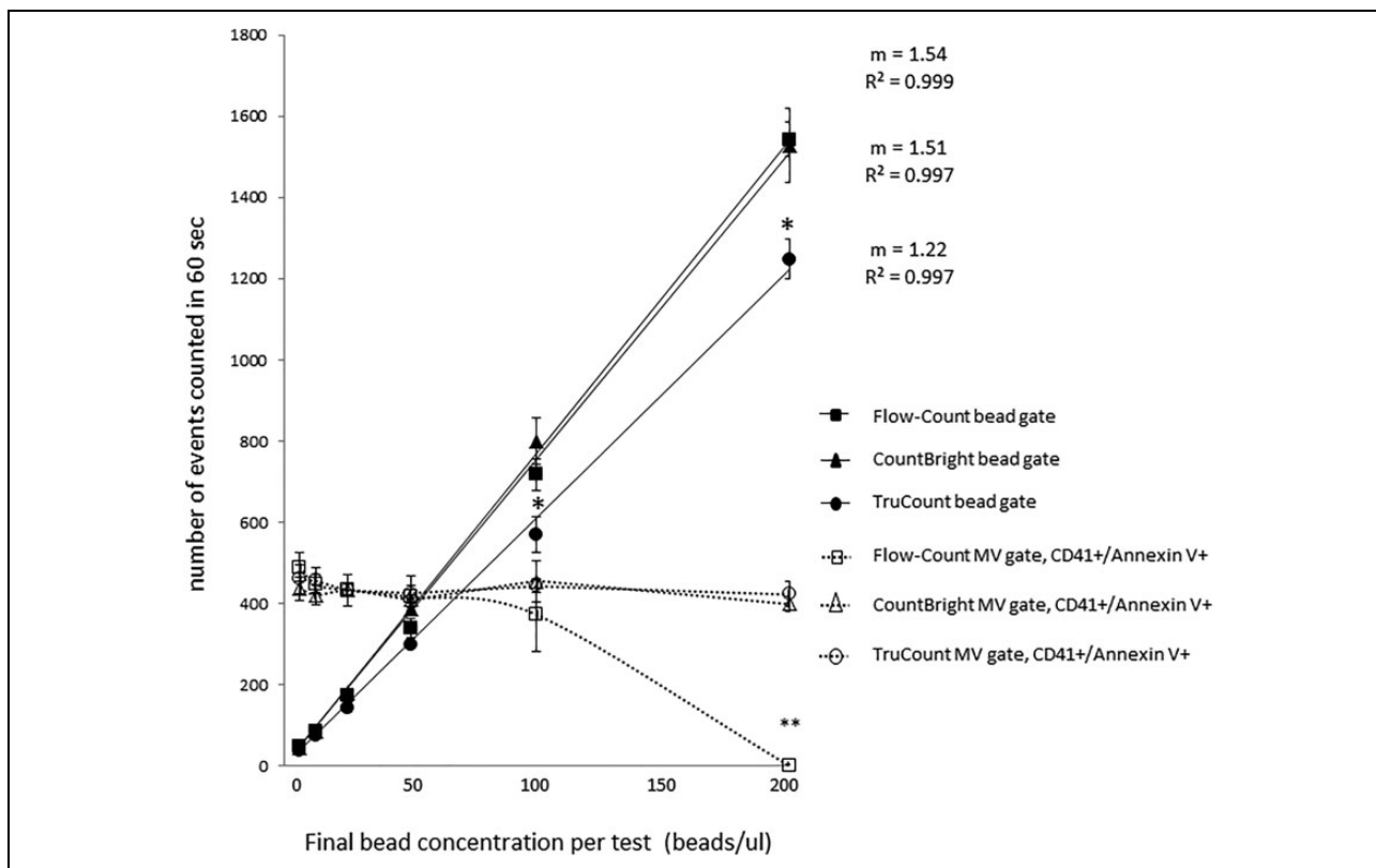
Figure 1. Correlation between the number of bead events counted versus added to each test and MV events counted using different brands of absolute counting beads. Solid lines and filled icons represent bead events, whereas dotted lines and outlined icons represent corresponding raw CD41 + /Annexin V + MV events detected by flow cytometry for each bead dilution. * p \leq 0.05 for TruCount versus CountBright and/or Flow-Count bead events; ** p \leq 0.001 for Flow-Count versus TruCount and/or CountBright MV events. MV: microvesicle.
