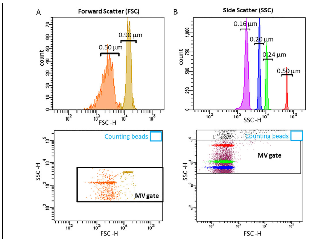
Figure 2. Flow cytometry resolution of sizing beads and MV gate settings using FSC versus SSC as the main size parameter. (a) The histogram in the top panel shows resolution of 0.5 \mu\text{m} (orange) and 0.9 \mu\text{m} (yellow) Megamix beads by FSC. The same beads are depicted in the dot plot below where the 0.9 \mu\text{m} bead cloud is used to set the MV gate. (b) The histogram in the top panel shows resolution of 0.16 \mu\text{m} (pink), 0.20 \mu\text{m} (blue), 0.24 \mu\text{m} (green) and 0.5 \mu\text{m} (red) Megamix-Plus SSC beads using FITC as the main parameter. The same beads are depicted in the dot plot below using SSC as the threshold to eliminate the 0.16 \mu\text{m} (pink) beads and use the 0.5 and 0.2 \mu\text{m} bead clouds to set the MV gate. The gate for capturing the counting beads is depicted in blue on both dot plots.
