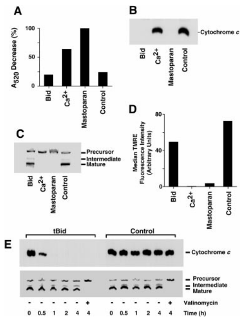
Figure 5. Mitochondria isolated from HL-60 cells retain protein import function and intact \Delta\Psi_m after cytochrome c release. Mitochondria (5 mg/ml as protein) were incubated in PT buffer, with the addition (as indicated) of 10 \mu\text{g/ml} tBid, 1 mM \text{CaCl}_2 , or 20 \mu\text{g/ml} mastoparan for 30 min at 22°C. (A) Mitochondrial swelling was assessed by comparing absorbance at 520 nm before and 25 min after the indicated additions were made. The A_{520} decrease produced by mastoparan was taken as 100%. 30 min after additions, aliquots were removed and analyzed for mitochondrial cytochrome c content (B) or import competence (C). 50 nM TMRE was added to the remaining samples, and (D) dye uptake was measured by flow cytometry after a further 10 min at 22°C. Finally, a second measurement of background fluorescence was made after valinomycin (1 \mu\text{M} ) was added to all samples. B shows the median fluorescence with this background subtracted. (E) HL-60 mitochondria remain import-competent for at least 3 h after complete cytochrome c release. HL-60 cell mitochondria (5 mg/ml protein) were incubated in PT buffer in the presence or absence of tBid (10 \mu\text{g/ml} ) as indicated. Aliquots of the reaction were taken at the indicated times and analyzed for cytochrome c content and import competence. As a control showing import dependence on \Delta\Psi_m , 1 \mu\text{M} valinomycin was added where indicated. Data are representative of three independent experiments.
