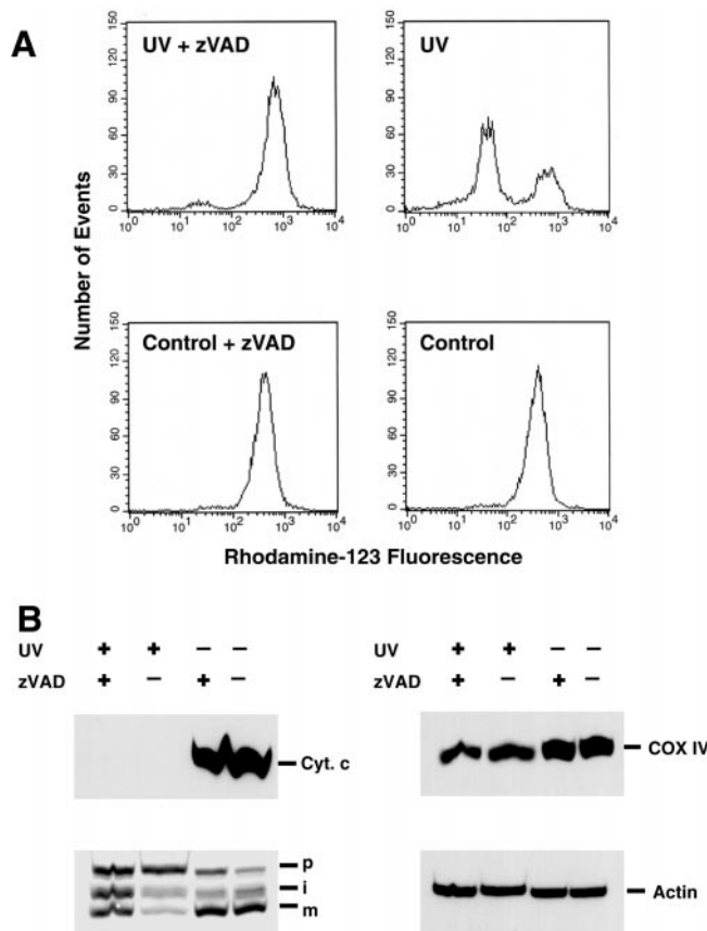
Figure 7. When caspases are inhibited, UV-irradiated HeLa cells display a complete loss of mitochondrial cytochrome c , but retain mitochondrial import function. (A) Loss of \Delta\Psi_m in apoptotic cells is blocked by caspase inhibition. HeLa cells were exposed to 180 mJ/cm 2 UVC light and further cultured for 8 h in medium with or without 100 \mu M zVAD-fmk as indicated. After this time, >50% of UV-treated cells showed an apoptotic phenotype in the absence of zVAD-fmk. Cells were harvested, and rhodamine-123 retention was measured by flow cytometry (10,000 events shown without gating). In the presence of zVAD-fmk, apoptotic cells retain \Delta\Psi_m . (B) Mitochondrial import competence is retained in the presence of zVAD-fmk. After flow cytometric analysis (A), the cells were permeabilized with digitonin and analyzed for cytochrome c content and import-competence. Cell pellets were extracted with NP-40 lysis buffer (150 mM NaCl, 1% NP-40, and 50 mM Tris-Cl, pH 8.0), and the protein content of the extract was determined by the Bradford assay. Finally, 50 \mu g of protein from each sample was subjected to SDS-PAGE and Western blotting. Quantitative analysis by phosphorimaging revealed 82 and 17% imported protein in the UV-treated samples with or without zVAD, respectively. Control samples gave 100 and 89% import, respectively (the control sample with zVAD was taken as 100%). Blots were stripped and reprobbed with antibodies to COX-IV and actin to demonstrate equal gel loading.
