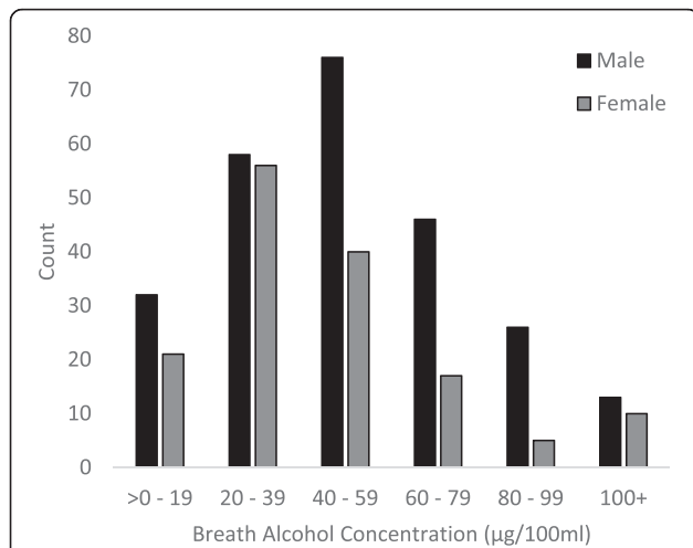
Fig. 1 Histogram of breath alcohol scores for all respondents who yielded a BrAC greater than zero and were included in the judgement analyses (N = 400)
