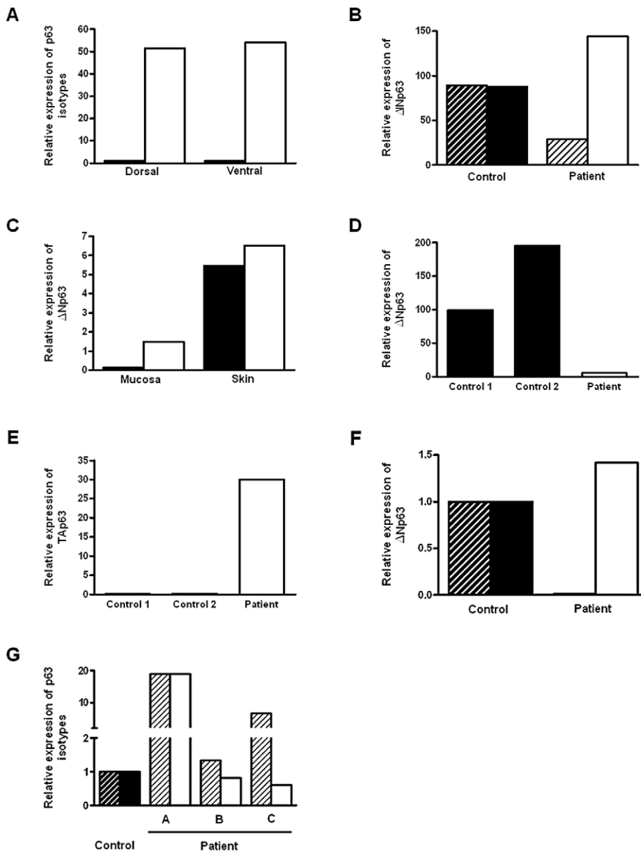
Figure 1. Expression of p63 isoforms in BEEC patient tissue and controls. (A) Real-time qPCR of \Delta Np63 (white column) and TP63 (black column) expression dorsal and ventral foreskin from normal control (2 yr. male). (B) Real time qPCR of \Delta Np63 expression dorsal (black hatched column) and ventral foreskin (white column) from a BEEC patient. (C) Real-time qPCR of \Delta Np63 expression in from BEEC patient (8 yr. male) dorsal (black column) and ventral (white column) foreskin mucosa and skin. (D) Real-time qPCR showing reduced \Delta Np63 mRNA expression in BEEC bladder epithelium compared with 2 normal controls. (E) Increased TP63 mRNA expression in BEEC bladder epithelium compared with 2 normal controls. (F) Real-time qPCR showing reduced \Delta Np63 mRNA and increased TP63 mRNA expression in bladder mucosa from a Caucasian BEEC patient (<1 yr. male) compared with normal controls (normalized to 1). (G) Real-time qPCR showing \Delta Np63 and TP63 mRNA expression in bladder mucosa from a three Caucasian BEEC patients (A, 13 yr. male; B, 14 yr. female; C, 6 yr. male) compared with normal controls (normalized to 1). doi:10.1371/journal.pgen.1003070.g001
