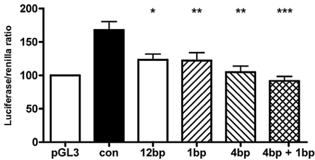
Figure 3. Indel polymorphisms decrease transcriptional efficiency. Luciferase assay of \Delta Np63 promoters with various indel polymorphisms transfected into human embryonic kidney (HEK-293) cells. Normal Control sequence (con), 12 base pair deletion (12 bp; rs6148242), 1 base pair insertion (1 bp, rs5855273), 4 base pair insertion (4 bp, ss#541028600). Data shown is the average of 8 experiments, each examined in triplicate. Data \pm SEM, * : p < 0.05 , ** p < 0.01 , *** : p < 0.001 , compared to normal control, One-way ANOVA, Bonferroni's Multiple Comparison test. doi:10.1371/journal.pgen.1003070.g003
