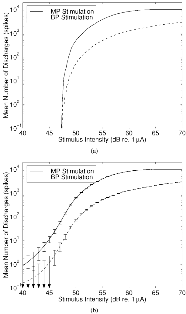
Fig. 5. Neural response versus stimulus intensity from a model of 10000 fibers in response to a single pulse for MP (solid line) and BP (dashed line) stimulation: (a) deterministic model and (b) stochastic model.
