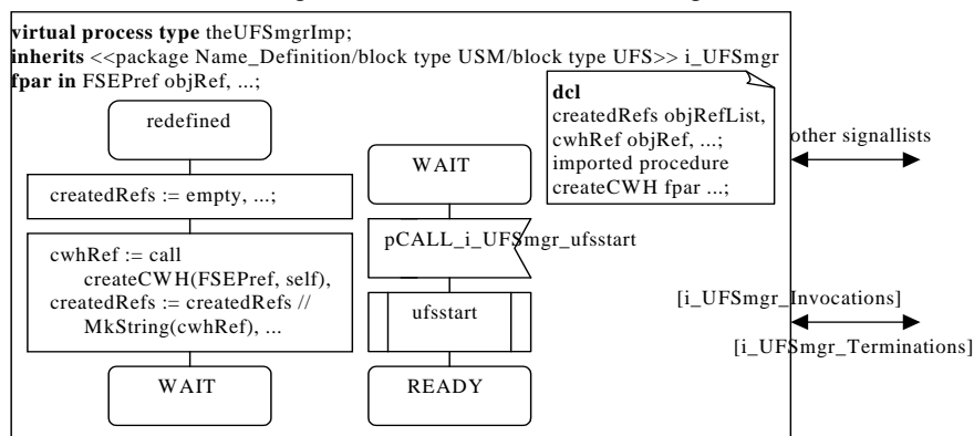
Figure 8 Structure of Basic UFSmgr.
