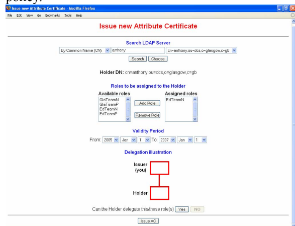
Figure 4: DIS Web Browser Interface
