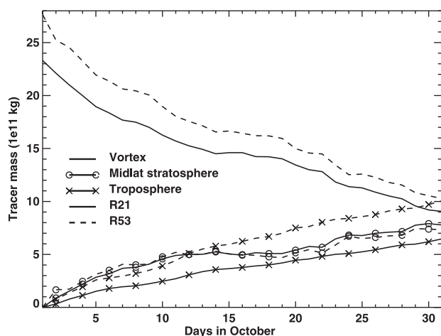
Figure 3. Temporal evolution of the total amount of tracer mass in the stratospheric vortex, the midlatitude stratosphere, and the troposphere in October 1994 for two different GASP resolutions R21 and R53.
