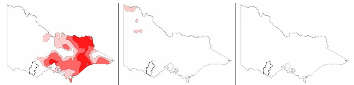
Figure 12: Incidence of 1 October to 31 March drought in Victoria, 2001-2012 (BoM, 2012). Corangamite Shire is illustrated by black outline in south-west. Pink: serious deficiency in rainfall (less than 10 th percentile). Light red: severe deficiency in rainfall (less than 5 th percentile). Solid red: lowest rainfall on record.
