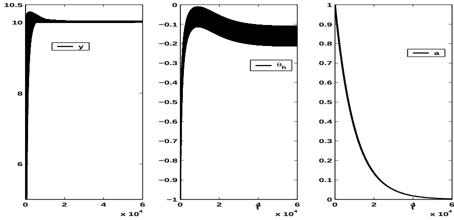
Figure 8: The performance of the proposed ES feedback scheme
