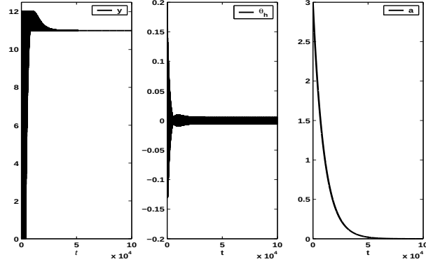
Figure 10: The output of the proposed ES feedback scheme
