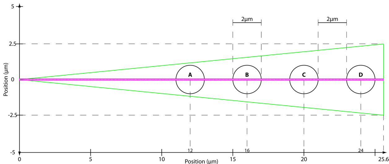
Fig 5. Simulation Geometry. The cell boundary is shown in green as an isosceles triangle 25.6μm wide and 5μm tall. The actin islands are shown as black circles with 1μm radii. As discussed in the text, unbound Rac1 molecules are free to diffuse throughout the cell and reflect off the cell boundary. Bound Rac1 molecules diffuse slower and are restricted to the inside of the island in which they are bound. We can individually set the K_D of each island thereby setting, on average, the percent of the total Rac1 population bound to each island. The 256 magenta boxes represent the (0.1\mu\text{m})^2 bins used to generate the intensity carpet; these bins do not affect the behavior of the molecules.
