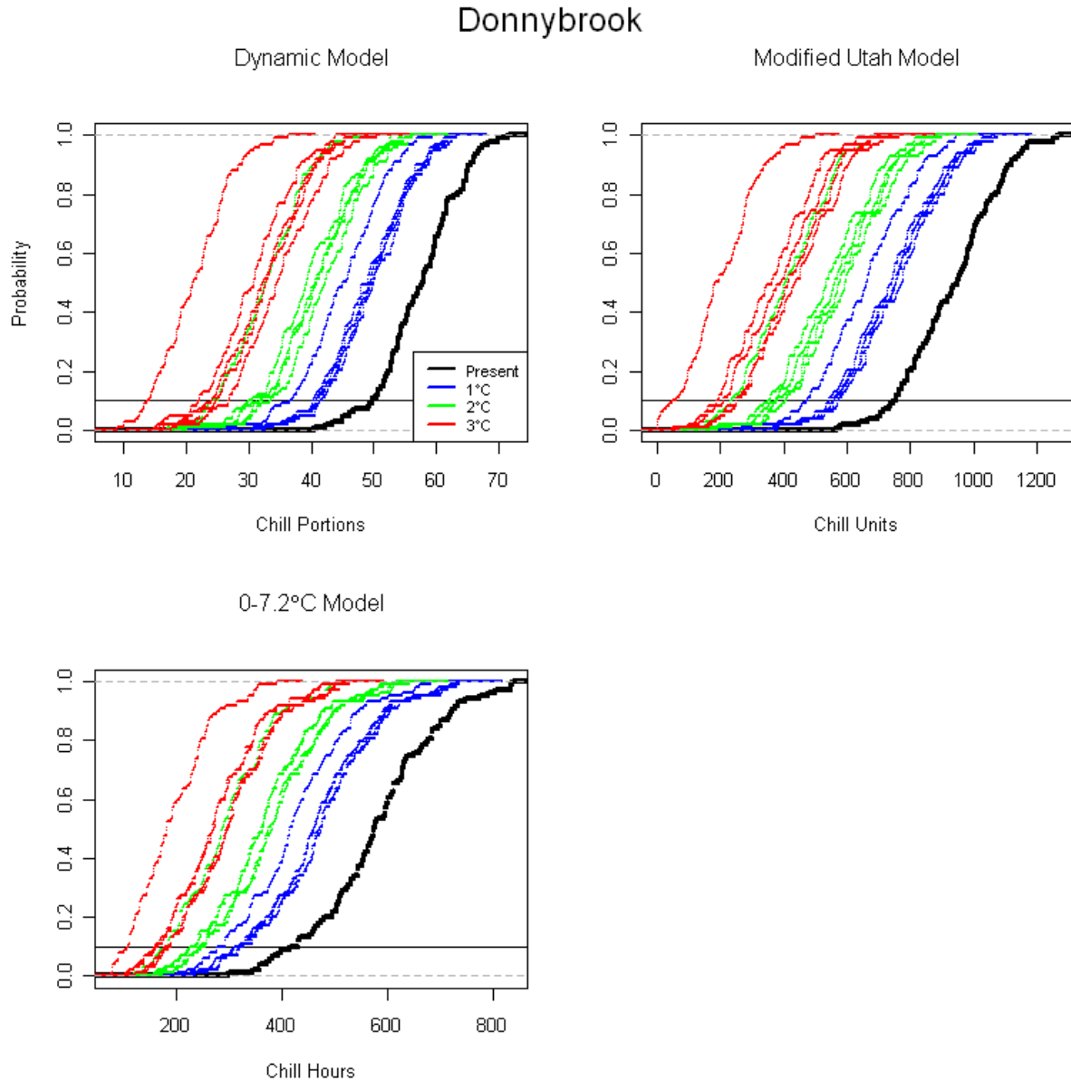
Figure 3 Cumulative distribution functions for projected chill conditions at Donnybrook (WA) according to the Dynamic, Modified Utah and 0-7.2°C models. Plots indicate current and localised change for 1, 2 and 3°C global average temperature increase for six AOGCMs. The solid horizontal line is the 10 th percentile representing ‘safe winter chill’
