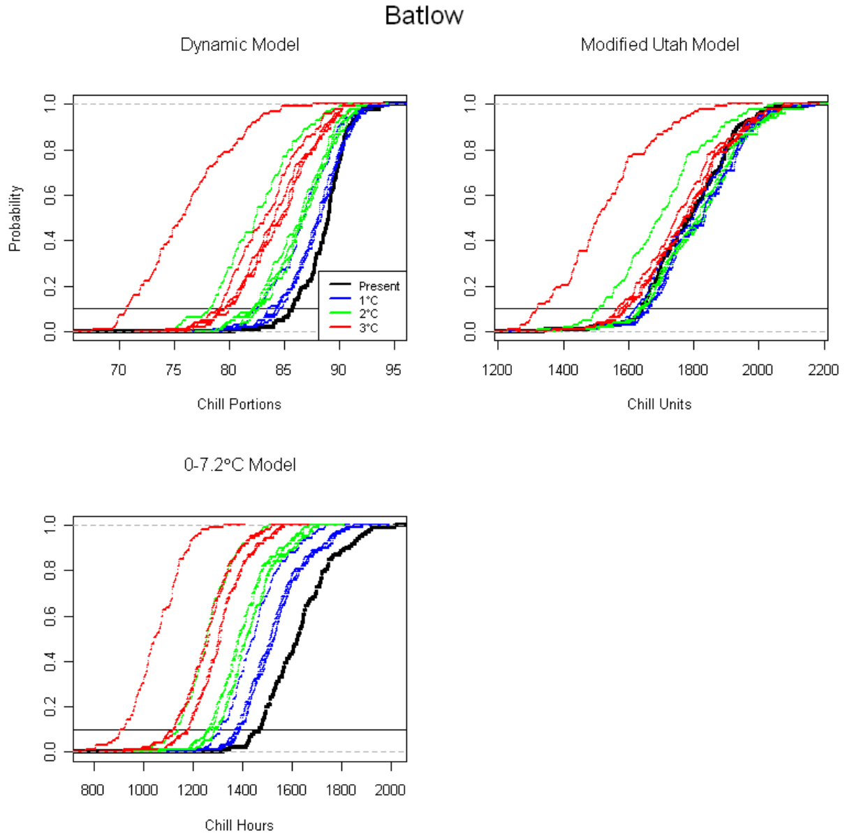
Figure 2 Cumulative distribution functions for projected chill conditions at Batlow (NSW) according to the Dynamic, Modified Utah and 0-7.2°C models. Plots indicate current and localised change for 1, 2 and 3°C global average temperature increase for six AOGCMs. The solid horizontal line is the 10 th percentile representing ‘safe winter chill’.
