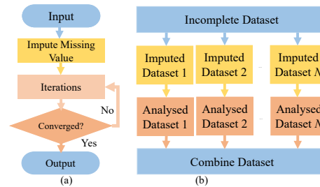
Fig. 3. A Schematics demonstration of the multiple Imputation, (a) represents Model-based Method and (b) represents Imputation-based Method.
