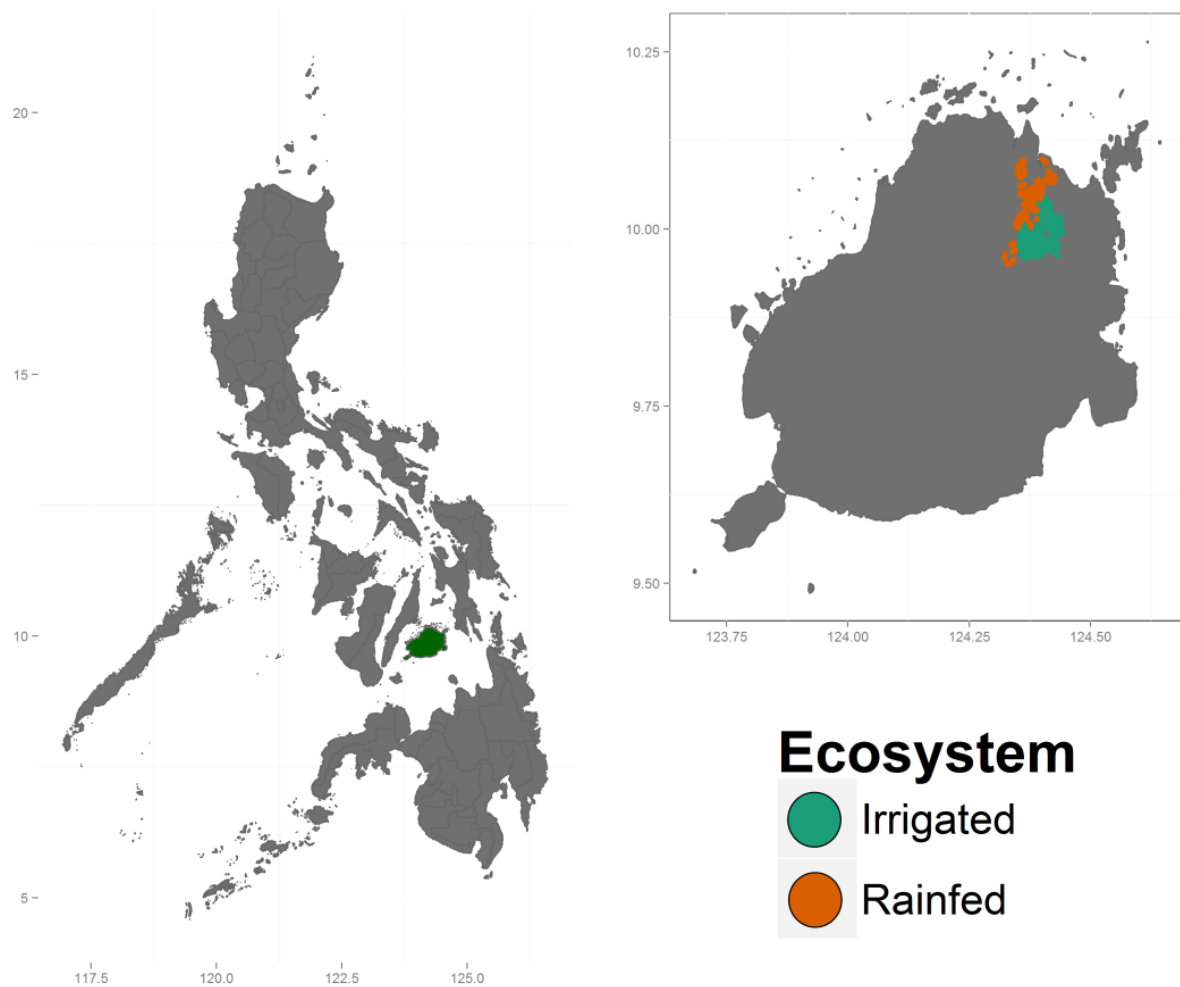
Fig. 1. Location of study sites designated by ecosystem.
