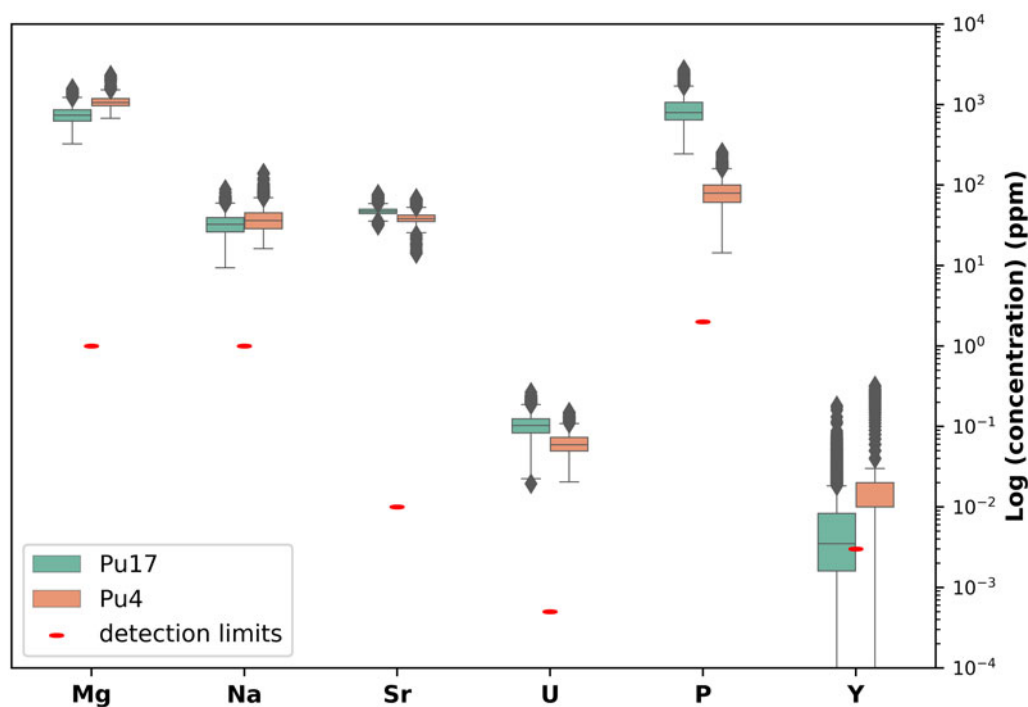
Figure 4. Boxplots showing the ranges of trace element concentration in the two studied stalagmites. The detection limit for each element is shown as a red dash.
