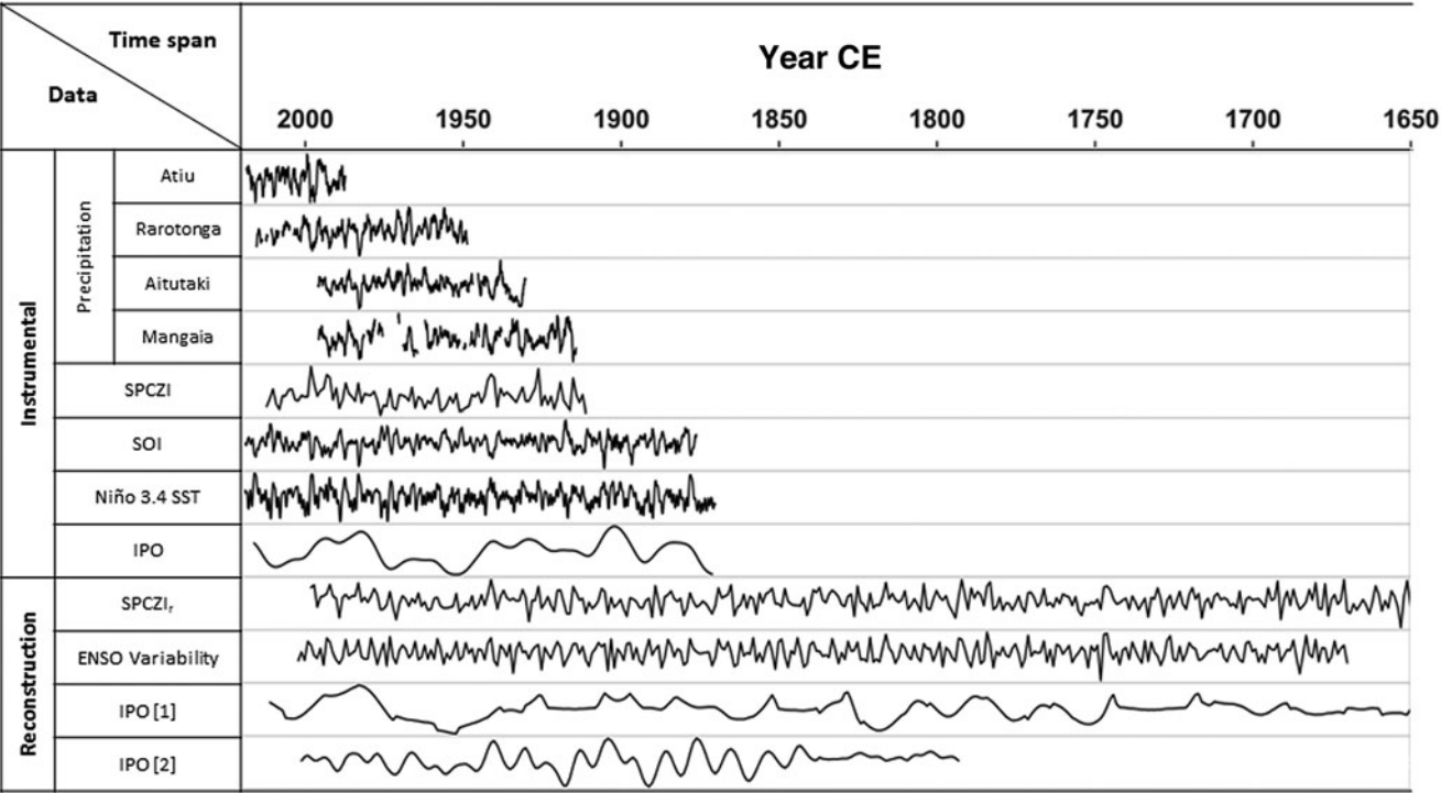
Figure 3. The instrumental and reconstructed climate data used in this study. ENSO = El Niño Southern Oscillation; IPO = Interdecadal Pacific Oscillation (IPO[1] data from Vance et al., 2022; IPO[2] data from Linsley et al., 2008); SOI = Southern Oscillation Index; SPCZI = South Pacific Convergent Zone Instrumental (from Higgins et al., 2020).
