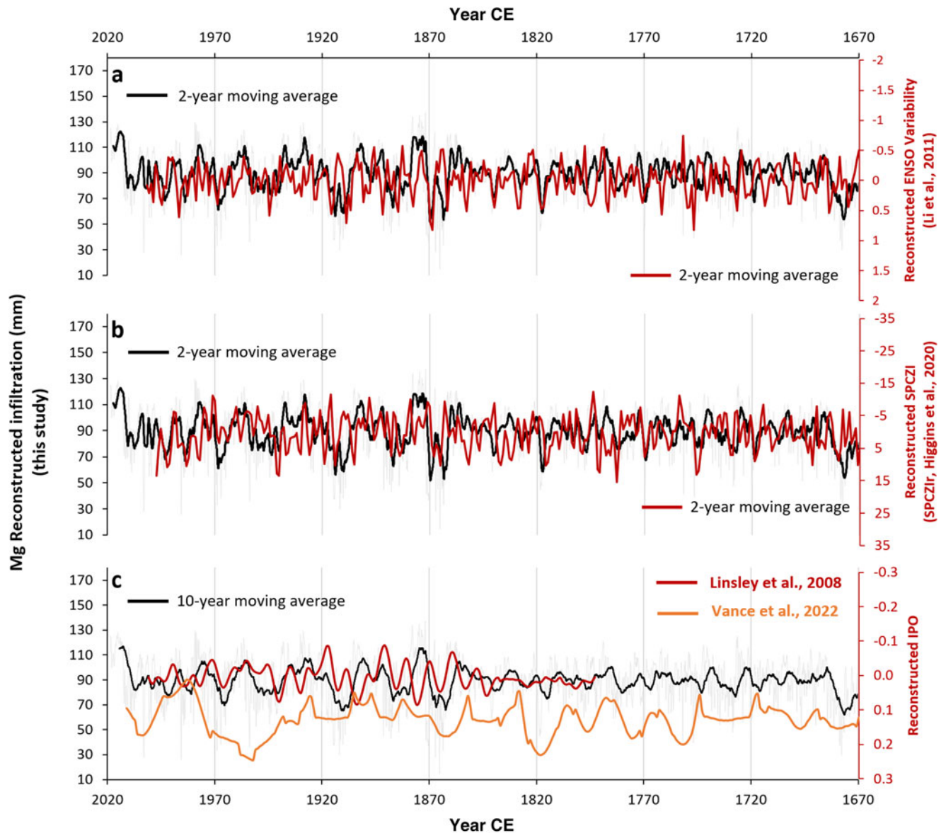
Figure 10. Infiltration derived from the time series of Mg in Pu17 compared with ENSO anomaly (Li et al., 2011), reconstructed SPCZI (SPCZI) (Higgins et al., 2020), and IPO (Linsley et al., 2008; Vance et al., 2022) as the main factors driving climate in the South Pacific. The figure shows that the reconstructed infiltration matches very well with these records, even though discrepancies exist because these are reconstructions and, undoubtedly, bear uncertainties.
