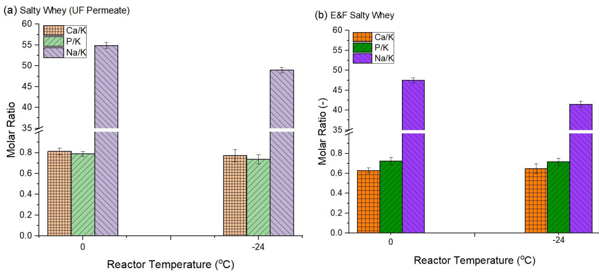
Figure 9: Molar ratio of calcium, phosphorus and sodium to potassium in the supernatant for (a) salty whey (UF permeate) and (b) evaporated and filtered salty whey samples at 0 and -24 °C.
