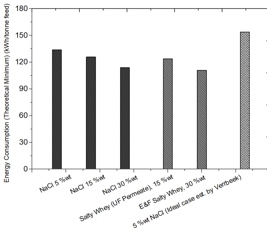
348 Figure 11: Theoretical minimum energy required for processing one tonne of different brine solutions 349 by EFC with 100% water and NaCl recovery. Data for the 5 wt% NaCl ideal case is reported by Verbeek 350 [23].
