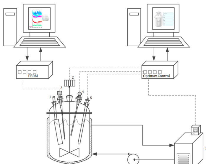
144 1 - Baffle blade, 2 - Impeller, 3 - FBRM, 4, HFCal, 5 - Temperature sensor, 6 - Water bath
