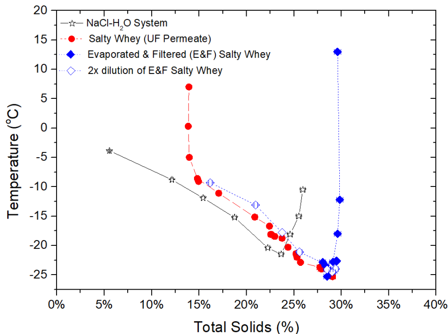
Figure 7: Phase diagram of aqueous sodium chloride solution, salty whey (UF permeate), E&F salty whey and diluted E&F salty whey. Lines are drawn to guide the eye.
