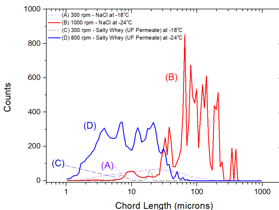
Figure 8: Chord length distribution of crystals for NaCl solutions and salty whey at -18^{\circ}\text{C} and -24^{\circ}\text{C} at different stirrer speeds.
