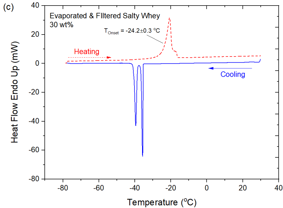
Figure 3: DSC thermograms (heat flow vs. temperature) measured during cooling (I and II) from 30°C to -80 °C and subsequent heating (III and IV) for (a) 13.8% NaCl in water, (b) salty whey (UF permeate) and (c) evaporated & filtered salty whey. The scanning rate was 3°C/min for both cooling and heating steps. The eutectic temperatures were determined to be -20.9 \pm 0.2 °C, -23.6 \pm 0.3 °C, and -24.2 \pm 0.3 °C for 13.8% NaCl in water, salty whey (UF permeate) and evaporated & filtered salty whey, respectively.
