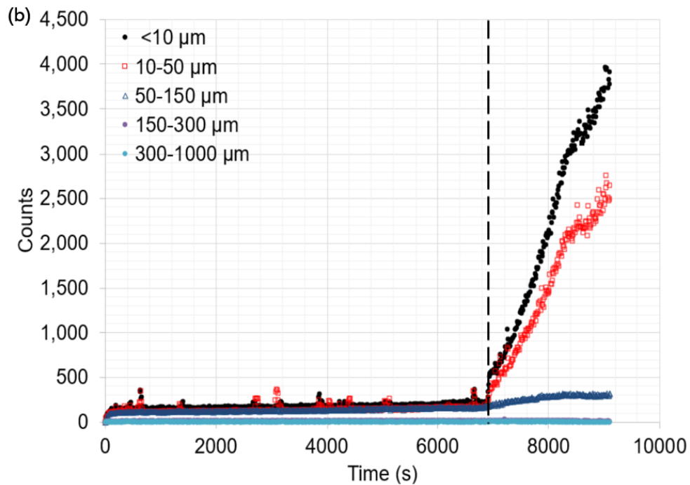
Figure 4: Temperature profile of the reactor (a) and counts of particles of various size (in \mu\text{m} ) within the reactor (b) during the crystallization of NaCl (18.7 wt%) using the OptiMax 1001 crystalliser. ( T_j : Jacket Temperature; T_r : Reactor Temperature). Crystallization occurs at 6800 s on the timeline.
