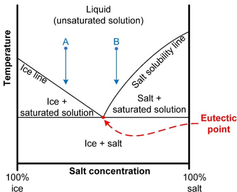
Figure 1: A typical phase diagram for aqueous salt solutions showing the Eutectic point [13]. (Copyright 2012, with permission from Elsevier.)
