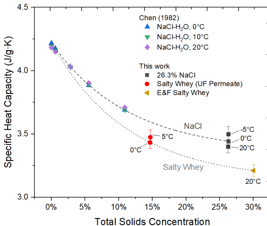
Figure 10: Specific heat capacity of NaCl solutions of different concentrations reported in the literature by Chen [26] and that of 26.3 wt% NaCl and salty whey samples measured in this work using the calorimetric probe (OptiMax™ HFCal). Lines are drawn to guide the eye.
