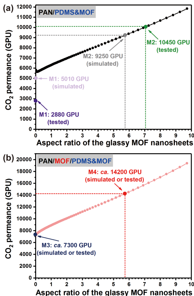
Figure 3. Comparison of tested and simulated CO 2 permeance of (a) M1: PAN/PDMS (with 0 v/v% amorphous MOF nanosheets loading) and M2: PAN/PDMS&MOF, and (b) M3: PAN/MOF/PDMS (with 0 v/v% amorphous MOF nanosheets loading) and M4: PAN/MOF/PDMS&MOF membranes with different amorphous MOF nanosheet aspect ratios in PDMS.
