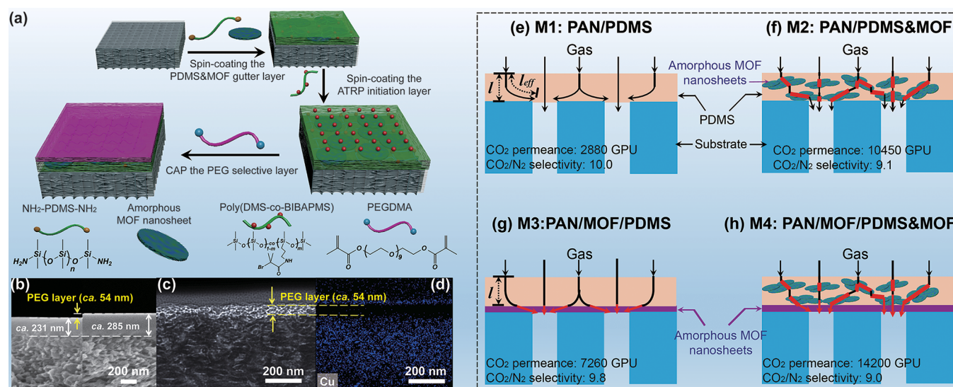
Figure 2. (a) Schematic illustration of the preparation of the TFC membranes by CAP technology. (b) Cross-sectional SEM image of the TFC membrane: (left) PDMS&MOF initiator layer and (right) the final TFC membrane. (c) Cross-sectional TEM image of the TFC membrane and (d) the corresponding Cu K energy-dispersive X-ray spectroscopy image. The yellow line marked areas in (c, d) represent the ultrathin PEG selective layer, and the blue color in (d) indicates the presence of amorphous MOF nanosheets in PDMS. (e) M1 ) Illustration of the geometric restriction effect on the gas diffusion length. A membrane with a gutter layer thickness of l will have an effective diffusion length ( l_{eff} ) larger than l due to the limited porous accessibility of the substrate. (f–h) Illustration of enhancing gas permeation rate via (f: M2 ) embedding ultrathin amorphous MOF nanosheets into PDMS matrix, (g: M3 ) introducing a porous amorphous MOF nanosheet layer between the PDMS gutter layer and substrate, and (h: M4 ) inserting a porous amorphous nanosheet layer between the PDMS&MOF gutter layer and substrate. The amorphous MOF nanosheet layer was coated onto a PAN substrate by vacuum filtration (CO 2 permeance: 38 000 GPU and N 2 permeance: 40 000 GPU), followed by spin-coating a PDMS or PDMS&MOF layer (2.0 w/v%, 1000 rpm, 10s).
