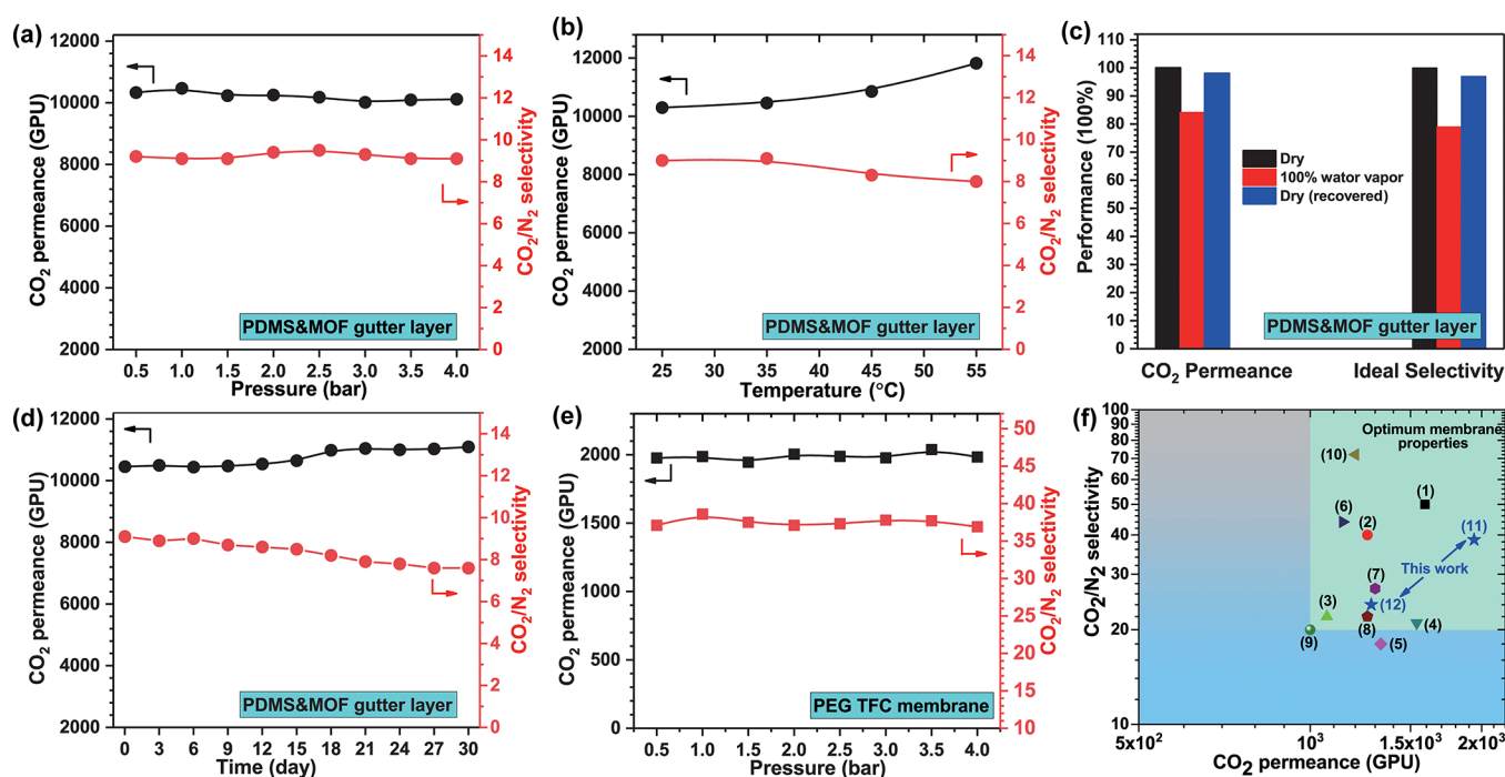
Figure 4. CO 2 /N 2 separation performance of PDMS&MOF gutter layer under variable conditions: (a) 0.5–4.0 bar, (b) 25–55 °C, (c) in the presence of 100% water vapor, and (d) long-term stability within 30 d. (e) The CO 2 /N 2 separation performance of complete PEG-based TFC membranes under a pressure range of 0.5–4.0 bar. (f) The CO 2 /N 2 selectivity vs CO 2 permeance plot comparing the performance of the prepared TFC membranes with other state-of-the-art TFC membranes reported in the literature. The region designated as the target performance area for postcombustion CO 2 capture was inferred from Merkel et al. 34 Further figure details are summarized in Table 1.
