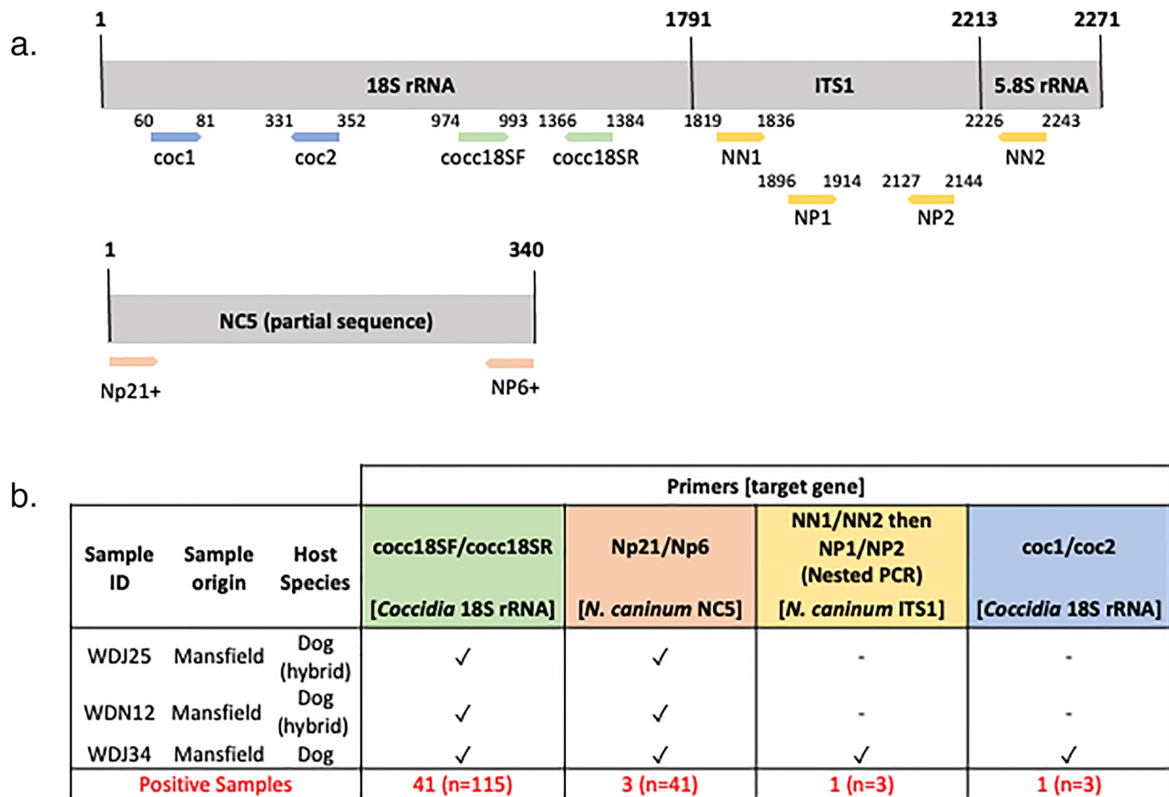
FIGURE 3 PCR amplification of Coccidia and Neospora DNA. (a) Schematic representation of the 18S rRNA, ITS1, 5.8S rRNA and Nc5 locus with relative location of oligonucleotide primers used in this study. Approximate primer position is provided based on Neospora caninum Liverpool strain genome annotation (GenBank accession number U16159) and partial Nc5 (GenBank accession number KP715563). (b) Summary of the PCR screens performed with Coccidia and N. caninum primers
