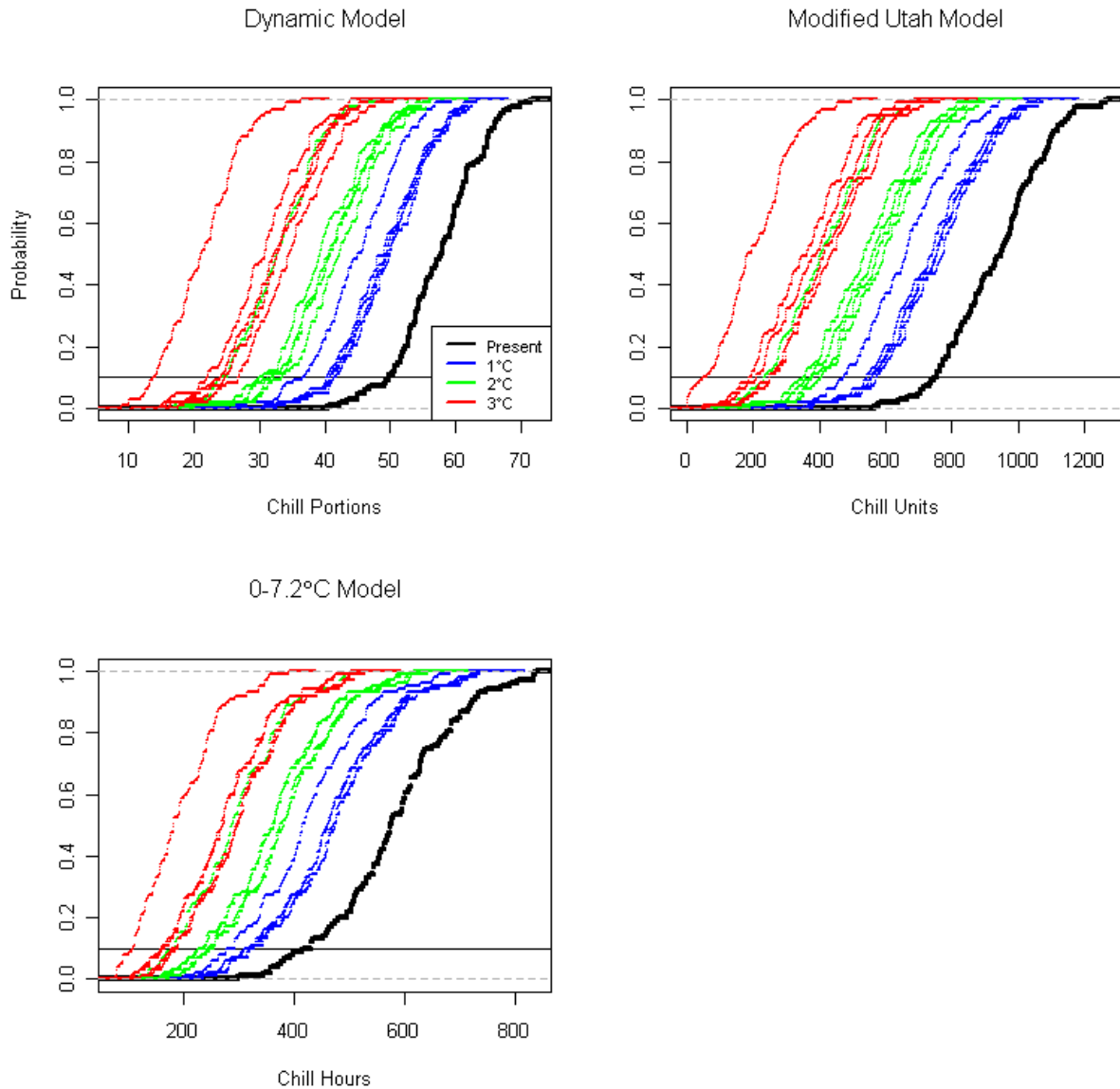
Figure 3 Cumulative distribution functions for projected chill conditions at Donnybrook (WA) according to the Dynamic, Modified Utah and 0-7.2°C models. Plots indicate current and localised change for 1, 2 and 3°C global average temperature increase for six AOGCMs. The solid horizontal line is the 10 th percentile representing ‘safe winter chill’
