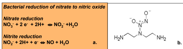
Figure 1: (a) Bacterial nitrate reduction generates nitric oxide, (b) The nitric oxide donor (Z)-1-[N-(2-aminoethyl)-N-2-aminoethyl]amino]dizen-1-ium1,2-diolate (DETA/NO•)
