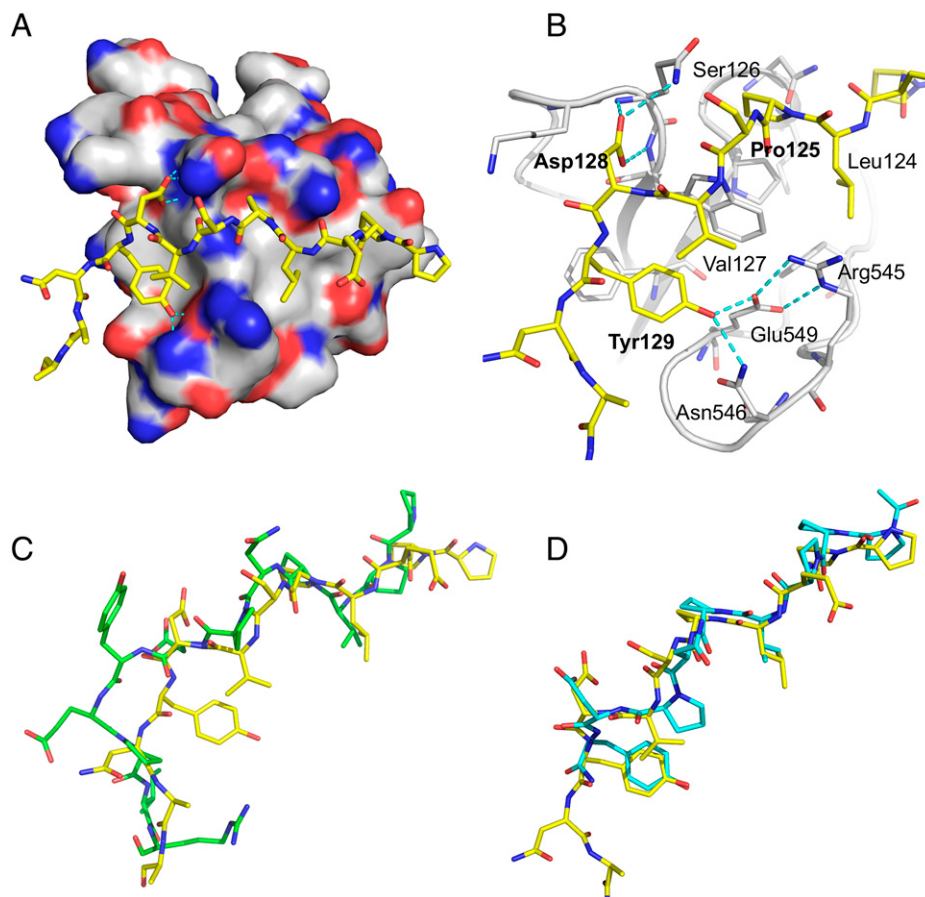
Fig. 3. Crystal structure of Eps8 SH3 domain with the NleH PPELPSPVDYNSL peptide. A. The PxxDY peptide binds in a shallow canyon on SH3 surface. The SH3 surface is colored by atom type: N, blue; O, red; C, white. The peptide is shown in a stick mode with the C atoms colored yellow. The charge and spatial complementarity between the SH3 domain and the NleH1 peptide is visible. Cyan dashed lines indicate hydrogen bonds. B. Closeup of the peptide-SH3 contacts. Asp and Tyr sidechains form hydrogen bonds (dashed lines) to the sidechain and mainchain atoms of SH3 residues. The P, D, and Y residues of the PxxDY motif are labeled in bold. C. PxxDY peptide bound to Eps8L1 SH3 (NMR structure 2ROL, green carbons) and NleH peptide bound to Eps8 SH3 (this structure, yellow carbons) based on the superposed SH3 domains. The key tyrosine points in different directions in the two structures D. PxxDY peptides from Nck1 (X-ray structure 5QU2, green carbons) and Eps8 SH3 domains (this structure, yellow carbons) based on the superposition of the corresponding SH3 domains. The conformations of these two peptides are very similar despite several amino acid differences.
