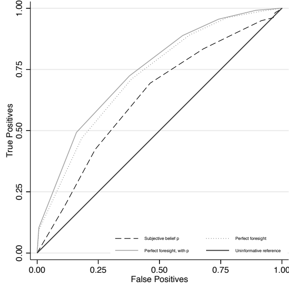
Figure 3: ROC FOR PREDICTING POST-SECONDARY EDUCATION COMPLETION AFTER AT LEAST TEN YEARS
