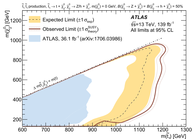
Fig. 10 Exclusion limits at 95% CL on the masses of the \tilde{t}_1 and \tilde{\chi}_2^0 , for a fixed m(\tilde{\chi}_1^0) = 0 GeV, assuming \mathcal{B}(\tilde{\chi}_2^0 \rightarrow Z\tilde{\chi}_1^0) = 0.5 and \mathcal{B}(\tilde{\chi}_2^0 \rightarrow h\tilde{\chi}_1^0) = 0.5 . The dashed line and the shaded band are the expected limit and its \pm 1\sigma uncertainty, respectively. The thick solid line is the observed limit for the central value of the signal cross-section. The expected and observed limits do not include the effect of the theoretical uncertainties in the signal cross-section. The dotted lines show the effect on the observed limit of varying the signal cross-section by \pm 1\sigma of the theoretical uncertainty. Results are compared with the observed limits obtained by the previous ATLAS search in Ref. [20]
