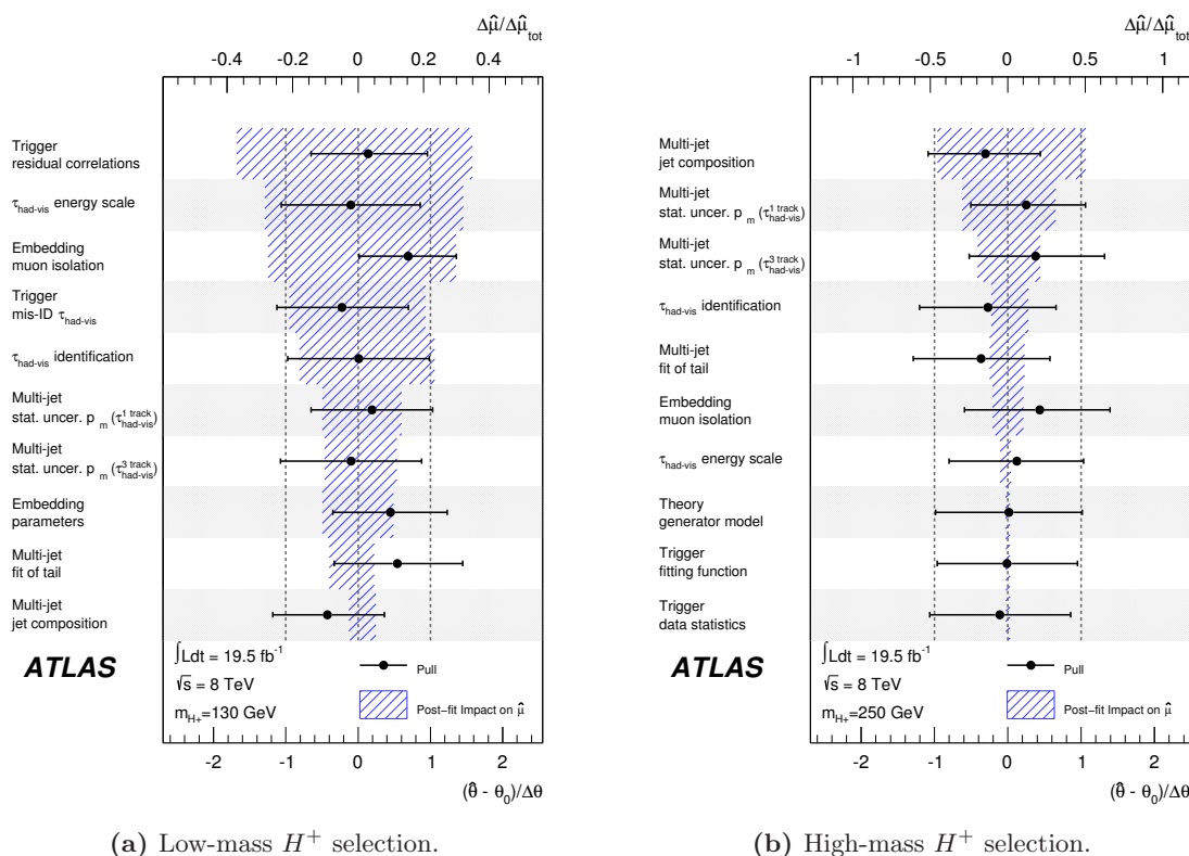
Figure 5. Impact of systematic uncertainties on the final observed limits for (a) m_{H^+} = 130 \text{ GeV} and (b) m_{H^+} = 250 \text{ GeV} . The systematic uncertainties are ordered (top to bottom) by decreasing impact on the fitted signal strength parameter. The dots, which refer to the bottom horizontal axis, show how each fitted nuisance parameter, \hat{\theta} , deviates from its nominal value, \theta_0 , in terms of standard deviations with respect to its nominal uncertainty, \Delta\theta . The solid lines indicate the post-fit uncertainties of each nuisance parameter, also relative to their nominal values. The hatched band, referring to the top horizontal axis, shows the deviations of the fitted signal-strength parameter after changing a specific nuisance parameter upwards or downwards by its post-fit uncertainty ( \Delta\hat{\mu} ) as a fraction of the total uncertainty of the fitted signal-strength parameter ( \Delta\hat{\mu}_{\text{tot}} ).
