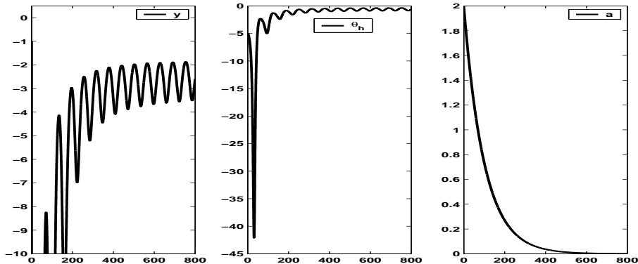
Figure 5: The output of the proposed extremum seeking feedback scheme, initial condition b
