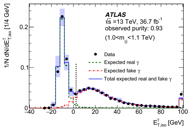
Fig. 2 Distribution of E_{T,iso}^{\gamma} = E_{T,iso} - 0.022 \times E_T^{\gamma} for the photon candidates in events with 1.0 < m_{\gamma j} < 1.1 TeV, and the comparison with the result of the template fit. Real- and fake-photon components determined by the fit are shown by the green dashed and red dot-dashed histograms, respectively, and the sum of the two components is shown as the solid blue histogram. The blue band shows the systematic uncertainties in the real- plus fake-photon template. The last bin of the distribution includes overflow events. The vertical dashed line corresponds to the isolation requirement used in the analysis. The photon purity determined from the fit for the selected sample in the 1.0 < m_{\gamma j} < 1.1 TeV mass range is 93%
