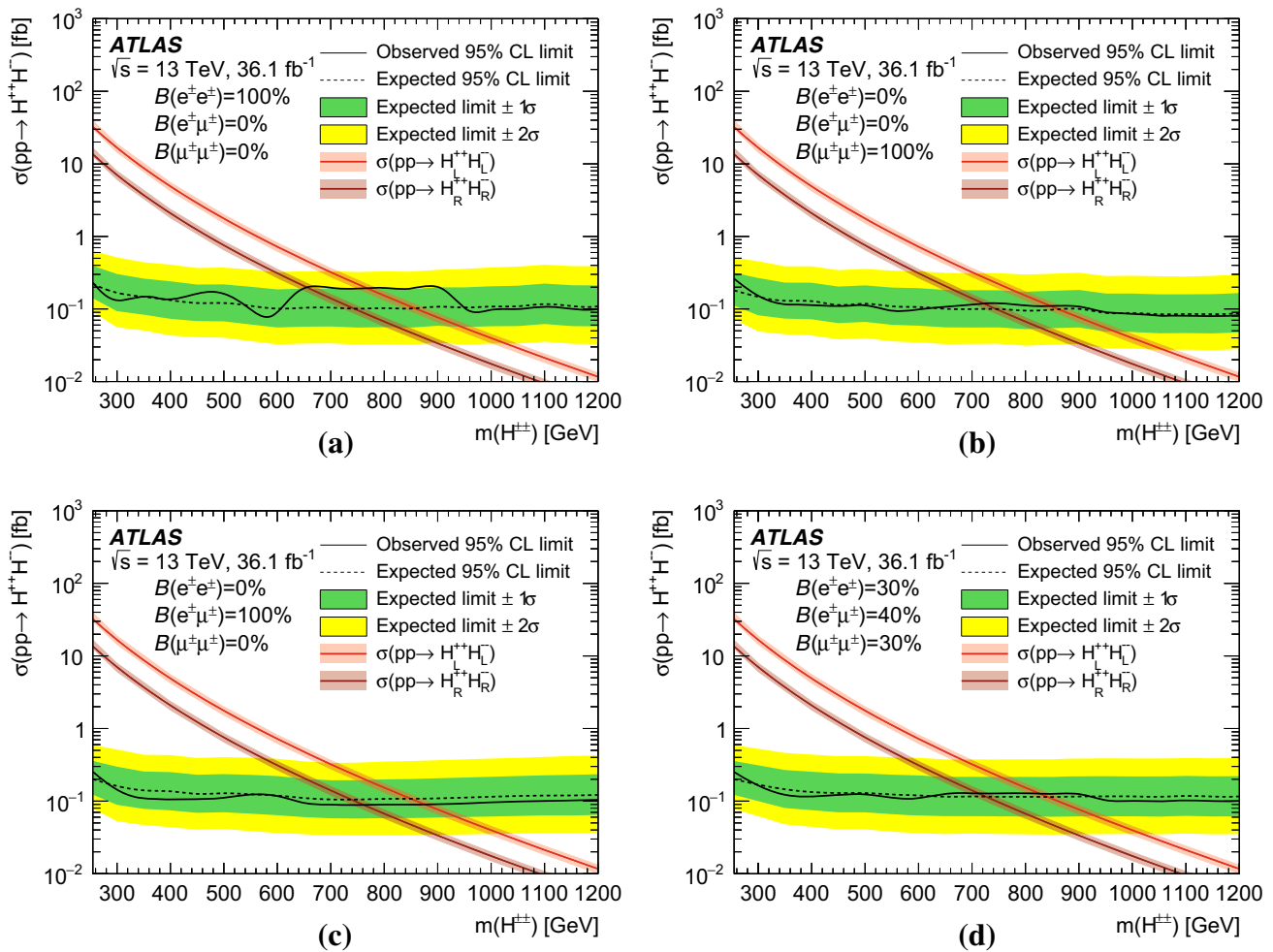
Fig. 10 Upper limit on the cross-section for pp \rightarrow H^{\pm\pm} H^{\mp\mp} for several branching ratio values presented in the form B(ee)/B(e\mu)/B(\mu\mu) : a 100%/0%/0%, b 0%/0%/100%, c 0%/100%/0%, and d
