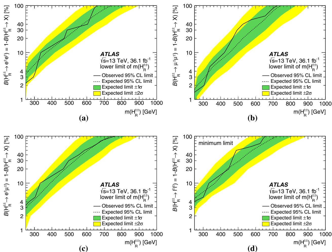
Fig. 14 Lower limit on the H_R^{\pm\pm} boson mass as a function of the branching ratio B(H_R^{\pm\pm} \rightarrow \ell^\pm \ell^\pm) . Several cases are presented: a H_R^{\pm\pm} decays only into electrons and “X”, b H_R^{\pm\pm} decays only into muons and
