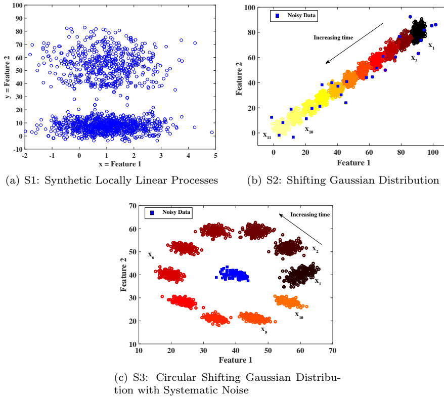
Figure 2: Scatter plots of three synthetic datasets. S2 and S3 show the progression of time with colors (depicted by an arrow), starting with black and becoming lighter with time.
