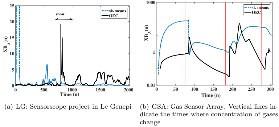
Figure 9: The XB_\lambda(n) index over the real-life datasets. The y-axis of GSA plot is shown in logarithmic scale.
