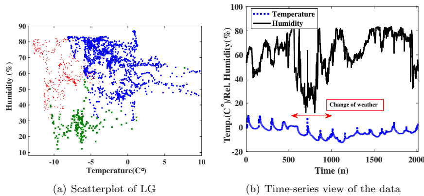
Figure 3: Scatterplot and time-series views of the LG data. The scatterplot shows three expected clusters.
