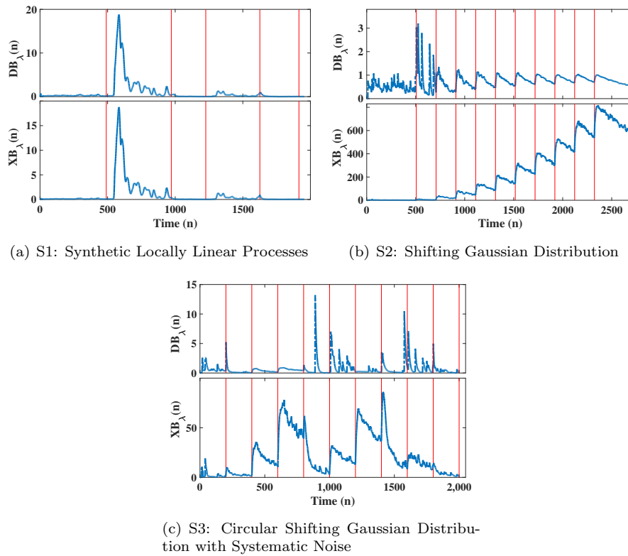
Figure 5: Values of XB_\lambda(n) and DB_\lambda(n) , \lambda = 0.9 , for sk-means. The vertical lines (red) are times when a change occurs in the dataset.
