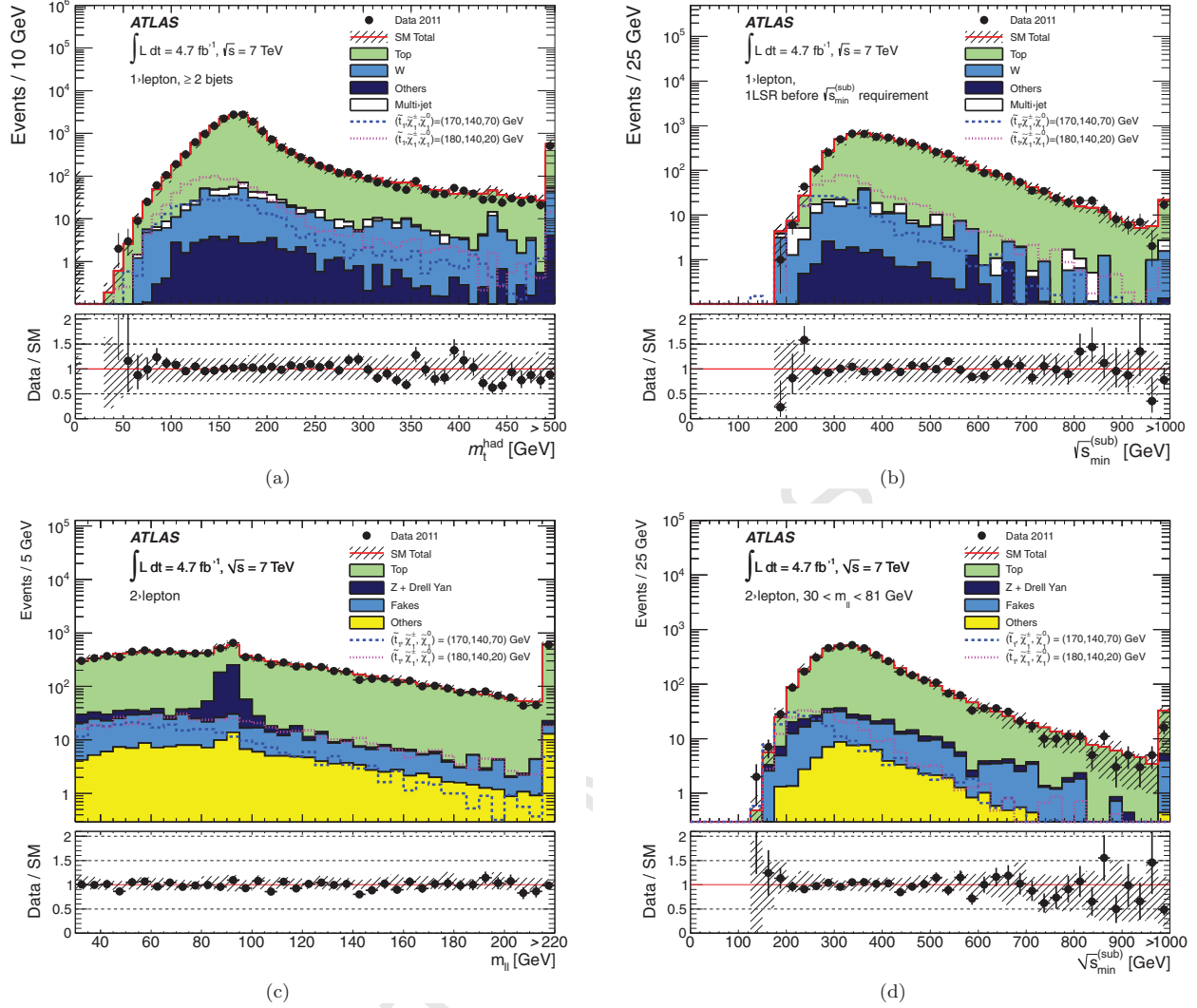
Figure 1: The 1-lepton channel m_t^{\text{had}} distribution after all requirements except those on m_t^{\text{had}} and \sqrt{s}_{\min}^{(\text{sub})} (a), and the \sqrt{s}_{\min}^{(\text{sub})} distribution after all requirements except that on \sqrt{s}_{\min}^{(\text{sub})} (b). For the 2-lepton channel, the m_{\ell\ell} distribution is shown after all requirements except those on m_{\ell\ell} and \sqrt{s}_{\min}^{(\text{sub})} (c), and the \sqrt{s}_{\min}^{(\text{sub})} distribution, before the requirements on \sqrt{s}_{\min}^{(\text{sub})} itself (d). The last bin in each histogram contains the integral of all events with values greater than the upper axis bound. The hatched bands display the total uncertainties on the background expectation and the dashed lines show the expected distributions for two signal models. The bottom panels show the ratio of data to the expected background (points) and the total uncertainty on the background (hatched area).
