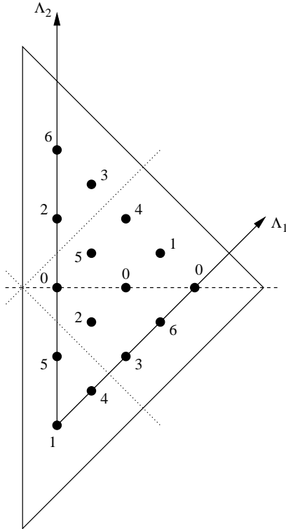
FIGURE 6.1. The integrable highest weights of C_2 at level 4 (shifted by \rho ) and the charges of the corresponding symmetry preserving D-branes. The charges take values mod 7. Note that the charges are negated (mod 7) under reflection about the dashed and dotted lines.
