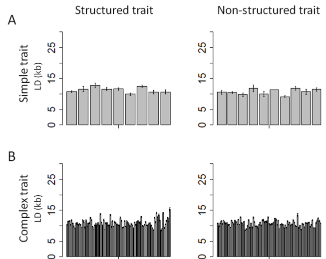
Figure 2. Estimation of LD around QTLs. Mean estimation of LD (in Kb) around the QTLs, calculated at r^2_{SV} = 0.2 between all loci in the 600 Kb neighborhood of each QTL locus on 3,000 individuals, for simple traits (A) and complex traits (B) on the 10 replicates of the simulation. The two figures on the left side represent LD around structured trait's QTLs and the other two figures around non-structured traits QTLs. QTL loci were ranked as a function of their effects from negative to positive values. Error bars were calculated with 95% confidence intervals on the estimates of the means.
