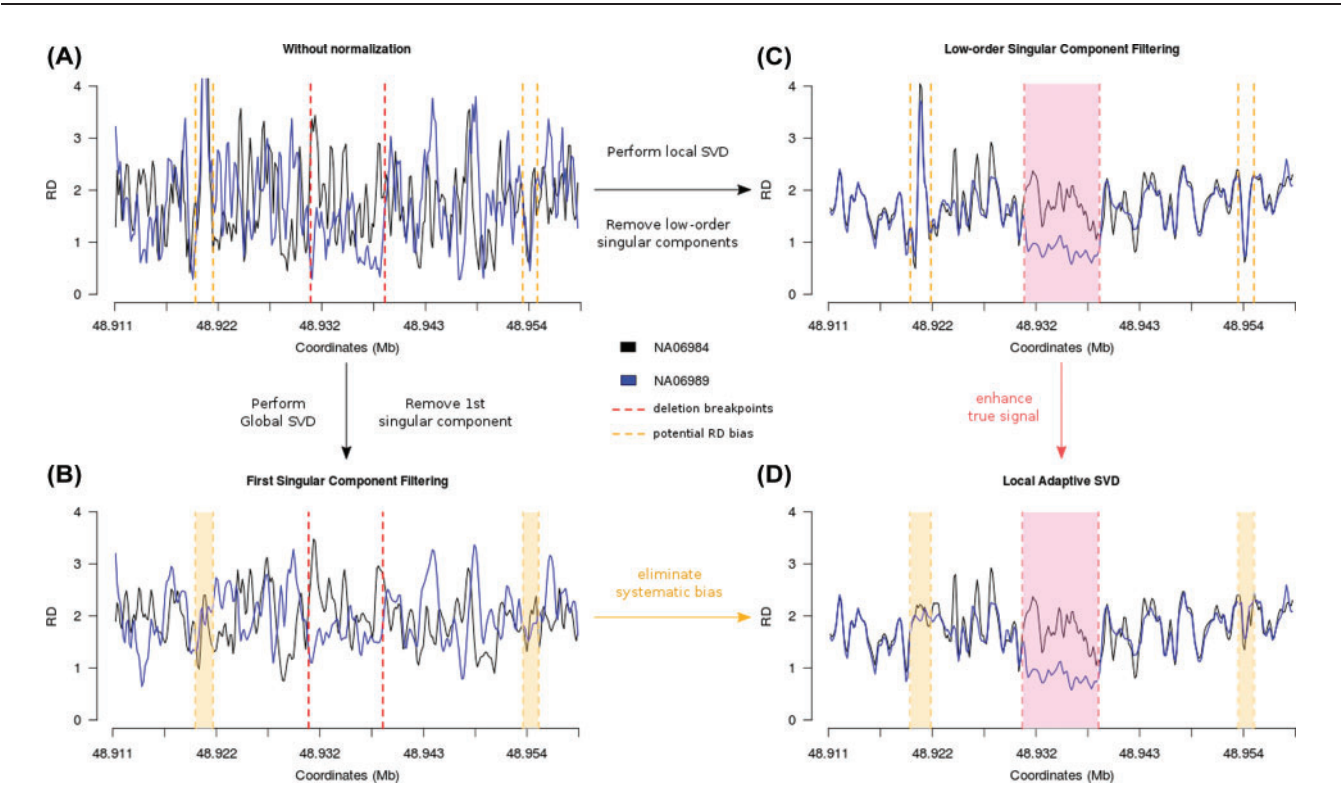
Fig. 2. Comparison of normalization techniques for two samples on chr6:48 911 000–48 959 000. The red dashed lines denote the breakpoints of a gold standard deletion that is present only in sample NA06989. (a) Raw RD data. The noisy nature of unnormalized RD makes the deletion difficult to detect in NA06989. The two regions denoted by the yellow dashed lines, show highly correlated RD profiles that most likely correspond to systematic bias. (b) Removing the first singular component mitigates the systematic bias, but also suppresses the signal of the true deletion. (c) Filtering low-order singular components de-noises the signal and enhances the true deletion but leaves systematic bias unaffected. (d) Our local adaptive SVD algorithm achieves the best results by combining the two approaches in one cohesive framework. The yellow shaded regions were normalized by filtering the first singular component (as in b) while the red shaded region was normalized by filtering low-order components (as in c)
