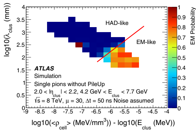
Fig. 10 Distribution of the likelihood \mathcal{P}_{\text{clus}}^{\text{EM}}(\rho_{\text{clus}}/E_{\text{clus}}^{\text{EM}}, \lambda_{\text{clus}}) for reconstructed topo-clusters to originate from an electromagnetic shower as a function of the shower depth \lambda_{\text{clus}} and the normalised cluster signal density \rho_{\text{clus}}/E_{\text{clus}}^{\text{EM}} , with \rho_{\text{clus}} = \langle \rho_{\text{cell}} \rangle being the energy-weighted average of \rho_{\text{cell}} . The shown distribution is determined as described in the text, in a selected bin of the cluster energy E_{\text{clus}}^{\text{EM}} and the cluster direction \eta_{\text{clus}} . The red line indicates the boundary of the \mathcal{P}_{\text{clus}}^{\text{EM}} > 50\% selection, below which the topo-cluster is classified as mostly electromagnetic (“EM-like”) and above which it is classified as mostly hadronic (“HAD-like”). The small EM-like area at the edge of the HAD-like region stems from neutral pions showering late. These areas are typical in regions of the detector where the second layer of the EM calorimeter is thinner and substantial parts of the shower are deposited in its last layer. The larger volume of the cells in this last layer leads to the reduced energy density while the position at the back of the EM calorimeter means a larger \lambda_{\text{clus}}
