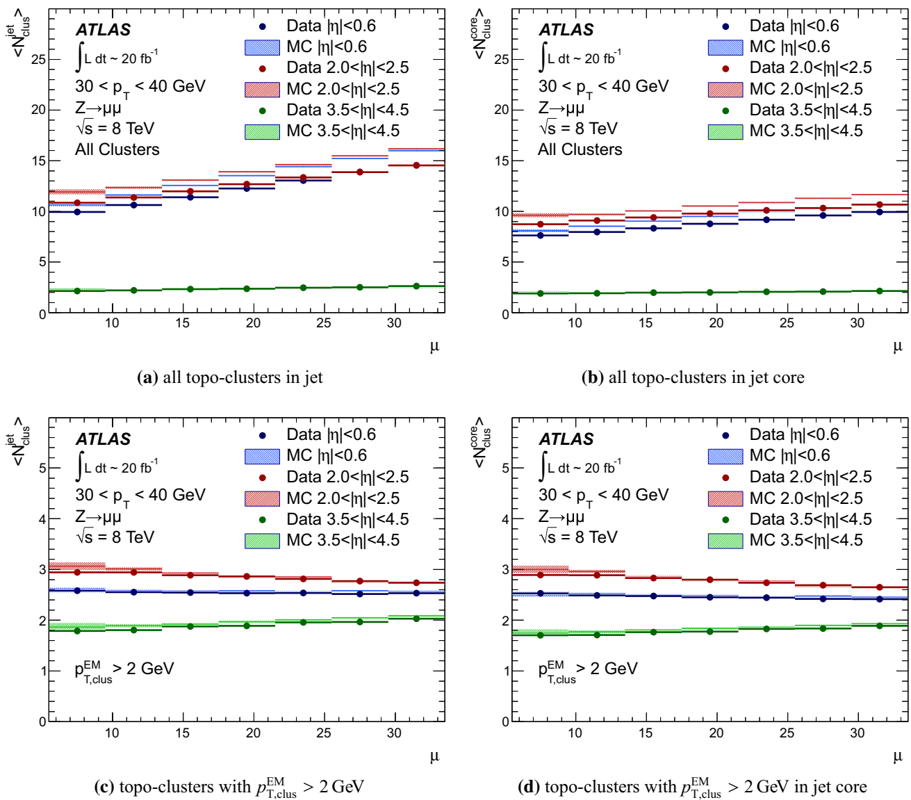
Fig. 33 The average number of topo-clusters \langle N_{clus}^{jet} \rangle in anti- k_t jets reconstructed with R = 0.4 within 30 \text{ GeV} < p_{T,jet}^{LCW+JES} < 40 \text{ GeV} as a function of \mu , in Z \rightarrow \mu\mu events in 2012 data and MC simulations (a). The pile-up dependence of the average number of topo-clusters \langle N_{clus}^{core} \rangle in the core of the jet, defined by the distance to jet axis \Delta R < 0.3 ,
