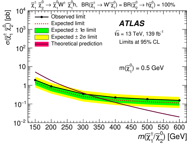
Figure 9. Expected and observed 95% CL exclusion upper limits on the production cross-section of \tilde{\chi}_1^\pm \tilde{\chi}_2^0 \rightarrow W^\pm \tilde{\chi}_1^0 h as a function of m(\tilde{\chi}_1^\pm/\tilde{\chi}_2^0) .
