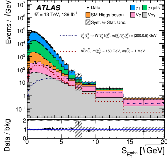
Figure 3. The distribution of S_{E_T^{\text{miss}}} after the selection of diphoton candidates with 120 < m_{\gamma\gamma} < 130 GeV. Expected distributions are shown for the \tilde{\chi}_1^\pm \tilde{\chi}_2^0 \rightarrow W^\pm \tilde{\chi}_1^0 h \tilde{\chi}_1^0 signal with m(\tilde{\chi}_1^\pm/\tilde{\chi}_2^0) = 200 GeV and m(\tilde{\chi}_1^0) = 0.5 GeV, and the h\tilde{G}h\tilde{G} signal with m(\tilde{\chi}_1^0) = 150 GeV and m(\tilde{G}) = 1 MeV. These overlaid signal points are representative of the model kinematics. The sum in quadrature of the MC statistical and experimental systematic uncertainties in the total background is shown as the hatched bands, while the theoretical uncertainties in the background normalisation are not included. The t\bar{t}\gamma and t\bar{t}\gamma\gamma processes have a negligible contribution and are not represented. Overflow events are included in the rightmost bin. The lower panel shows the ratio of the data to the background, called “bkg”.
