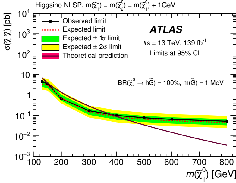
Figure 11. Expected and observed 95% CL exclusion upper limits on the higgsino production ( \tilde{\chi}\tilde{\chi} \equiv \tilde{\chi}_1^0\tilde{\chi}_2^0, \tilde{\chi}_1^0\tilde{\chi}_1^\pm, \tilde{\chi}_2^0\tilde{\chi}_1^\pm, \tilde{\chi}_1^\pm\tilde{\chi}_1^\mp ) cross-section for the h\tilde{G}h\tilde{G} signal model. As a function of the higgsino mass. The theoretical prediction includes the \tilde{\chi}_1^0\tilde{\chi}_2^0, \tilde{\chi}_1^0\tilde{\chi}_1^\pm, \tilde{\chi}_2^0\tilde{\chi}_1^\pm , and \tilde{\chi}_1^\pm\tilde{\chi}_1^\mp production modes, where \tilde{\chi}_1^\pm and \tilde{\chi}_2^0 promptly decay into the \tilde{\chi}_1^0 and particles that have too low momentum to be detected.
