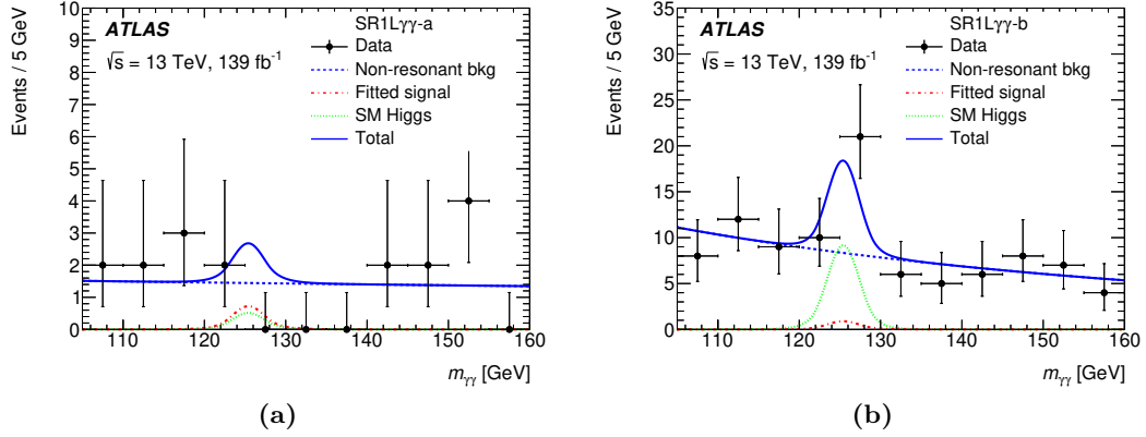
Figure 7. Diphoton invariant mass spectra and the corresponding fitted signal and background in the signal regions (a) ‘SR1L \gamma\gamma -a’ and (b) ‘SR1L \gamma\gamma -b’. The signal samples shown correspond to the \tilde{\chi}_1^\pm \tilde{\chi}_2^0 \rightarrow W^\pm \tilde{\chi}_1^0 h \tilde{\chi}_1^0 signal with m(\tilde{\chi}_1^\pm/\tilde{\chi}_2^0) = 200 GeV and m(\tilde{\chi}_1^0) = 0.5 GeV. The non-resonant background (dashed curve), the SM Higgs boson (dotted curve), and the signal (dash-dotted curve) are obtained from a signal-plus-background fit to the full m_{\gamma\gamma} spectrum in ‘SR1L \gamma\gamma -a’ (a) and ‘SR1L \gamma\gamma -b’ (b) separately. The total of these contributions is shown by the solid curves.
