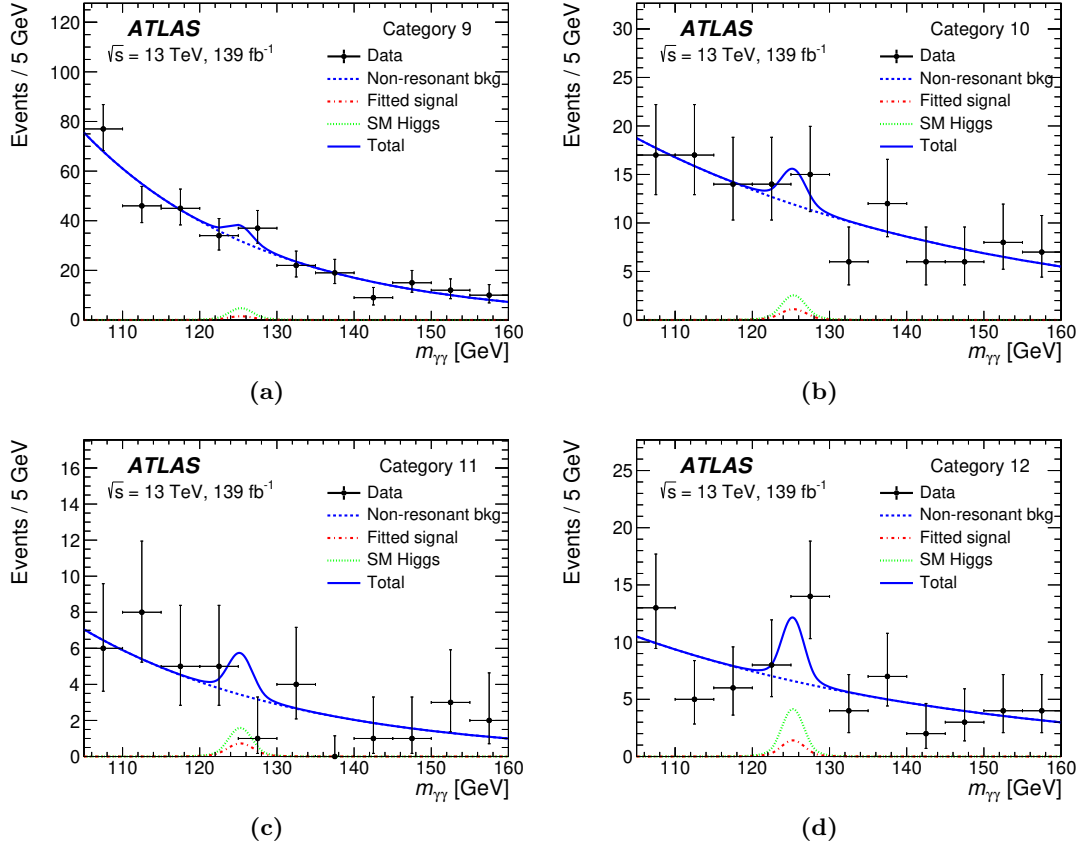
Figure 6. Diphoton invariant mass spectra and the corresponding fitted signal and background in the Rest categories (a) 9, (b) 10, (c) 11, and (d) 12. The signal samples shown correspond to the \tilde{\chi}_1^\pm \tilde{\chi}_2^0 \rightarrow W^\pm \tilde{\chi}_1^0 h \tilde{\chi}_1^0 signal with m(\tilde{\chi}_1^\pm/\tilde{\chi}_2^0) = 200 GeV and m(\tilde{\chi}_1^0) = 0.5 GeV. The non-resonant background (dashed curve), the SM Higgs boson (dotted curve), and the signal (dash-dotted curve) are obtained from a simultaneous signal-plus-background fit to the full m_{\gamma\gamma} spectrum for the 12 categories. The total of these contributions is shown by the solid curves.
