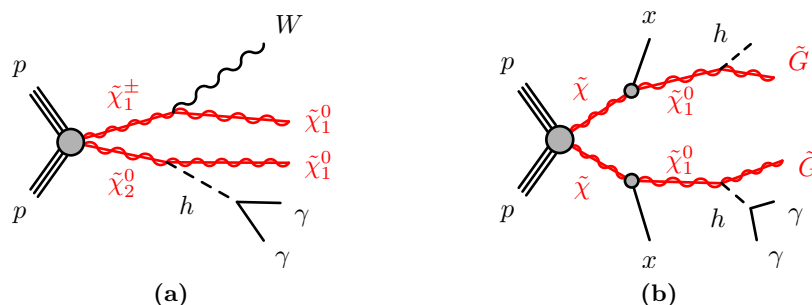
Figure 1. Signal diagrams illustrating (a) \tilde{\chi}_1^\pm \tilde{\chi}_2^0 production, and (b) a higgsino production mode from a GMSB model: \tilde{\chi}_1^0 \rightarrow h\tilde{G} . For \tilde{\chi}_1^\pm \tilde{\chi}_2^0 production, the lightest chargino ( \tilde{\chi}_1^\pm ) and next-to-lightest neutralino ( \tilde{\chi}_2^0 ) are nearly mass degenerate. In the higgsino models, the two lightest neutralinos, \tilde{\chi}_1^0 and \tilde{\chi}_2^0 , and the lightest chargino \tilde{\chi}_1^\pm are approximately mass degenerate, and the \tilde{\chi}_1^0 is the lightest of the four nearly degenerate higgsino states, x is the particle with low momentum from the promptly decay of \tilde{\chi}_1^\pm and \tilde{\chi}_2^0 .
