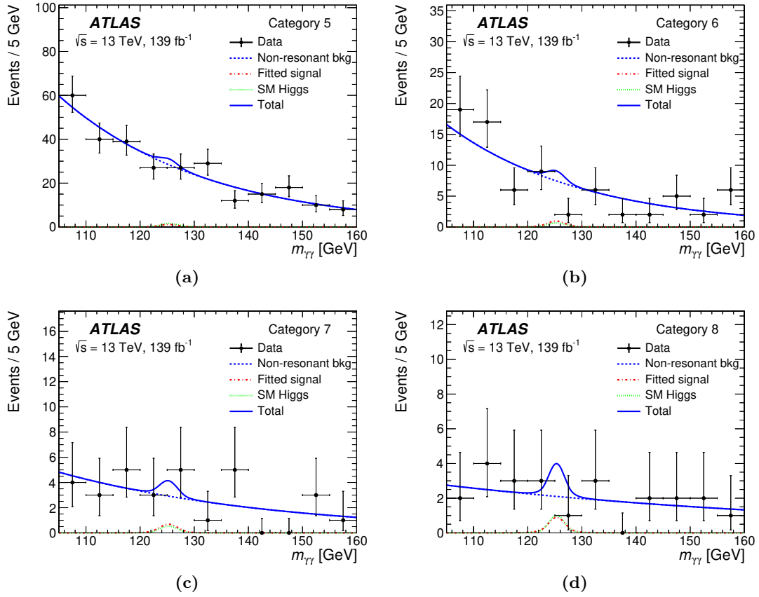
Figure 5. Diphoton invariant mass spectra and the corresponding fitted signal and background in the Hadronic categories (a) 5, (b) 6, (c) 7, and (d) 8. The signal samples shown correspond to the \tilde{\chi}_1^\pm \tilde{\chi}_2^0 \rightarrow W^\pm \tilde{\chi}_1^0 h \tilde{\chi}_1^0 signal with m(\tilde{\chi}_1^\pm/\tilde{\chi}_2^0) = 200 GeV and m(\tilde{\chi}_1^0) = 0.5 GeV. The non-resonant background (dashed curve), the SM Higgs boson (dotted curve), and the signal (dash-dotted curve) are obtained from a simultaneous signal-plus-background fit to the full m_{\gamma\gamma} spectrum for the 12 categories. The total of these contributions is shown by the solid curves.
