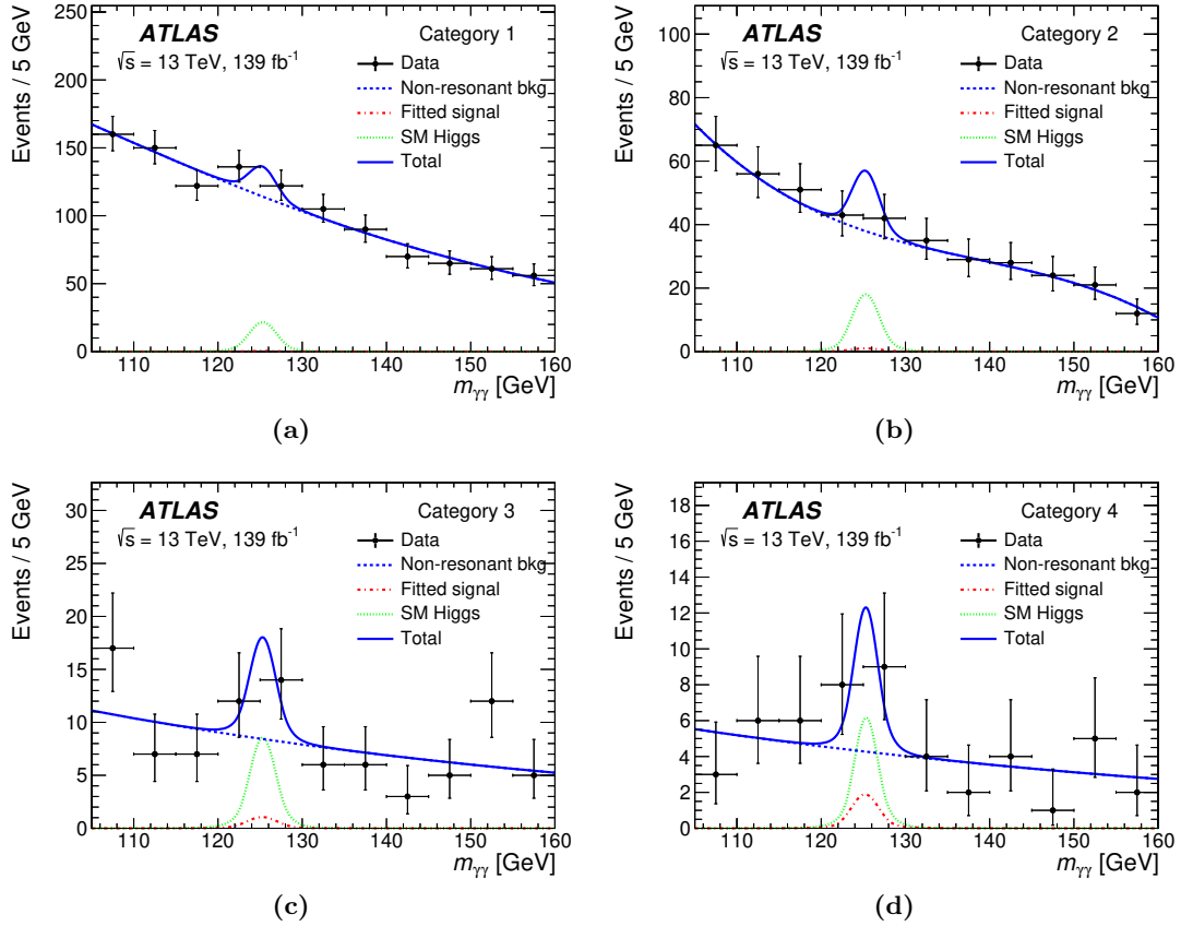
Figure 4. Diphoton invariant mass spectra and the corresponding fitted signal and background in the Leptonic categories (a) 1, (b) 2, (c) 3, and (d) 4. The signal samples shown correspond to the \tilde{\chi}_1^\pm \tilde{\chi}_2^0 \rightarrow W^\pm \tilde{\chi}_1^0 h \tilde{\chi}_1^0 signal with m(\tilde{\chi}_1^\pm/\tilde{\chi}_2^0) = 200 GeV and m(\tilde{\chi}_1^0) = 0.5 GeV. The non-resonant background (dashed curve), the SM Higgs boson (dotted curve), and the signal (dash-dotted curve) are obtained from a simultaneous signal-plus-background fit to the full m_{\gamma\gamma} spectrum for the 12 categories. The total of these contributions is shown by the solid curves.
