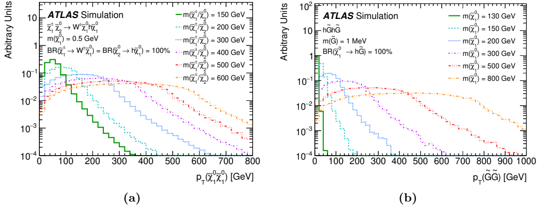
Figure 2. The p_T distribution of (a) the \tilde{\chi}_1^0 \tilde{\chi}_1^0 in W^\pm \tilde{\chi}_1^0 h \tilde{\chi}_1^0 production and (b) \tilde{G} \tilde{G} in h \tilde{G} h \tilde{G} production.
