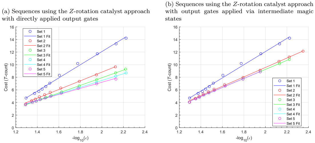
Figure 3: Cost-optimal sequence T -counts calculated using the Z -rotation catalyst approach plotted against synthesised target gate error rates of \epsilon . Each point is the result of averaging the T -count for implementing 5000 random target gate. The synthesis logical errors \epsilon are calculated using the trace distance (shown in Equation 8). The logical base gates for each set of base gates are specified in Equation 3. The corresponding linear best fit values for both plots are shown in Table 3. (a) A plot of sequence costs where base gates are assigned costs by assuming that all output gates are directly applied to target qubits. Base gate costs are calculated using Eq. 5 and enumerated in Table 1a. The reductions in scaling factors relative to Set 1 are 34 \pm 4\% , 43 \pm 2\% , 49 \pm 2\% , and 54 \pm 3\% for Set 2 , Set 3 , Set 4 , and Set 5 respectively, where uncertainties correspond to 95% confidence intervals. These correspond to synthesis cost savings in the limit of small \epsilon . (b) A plot of sequence costs where base gates are assigned costs by assuming that output gates are applied to |+\rangle states to form the corresponding intermediate magic states, gates are then applied by consuming the magic states via teleportation circuits. Base gate costs are calculated using Eq. 7 and enumerated in Table 1b. The reductions in scaling factors relative to Set 1 are 29 \pm 3\% , 31 \pm 3\% , 31 \pm 4\% , and 31 \pm 4\% for Set 2 , Set 3 , Set 4 , and Set 5 respectively, where uncertainties correspond to 95% confidence intervals. These correspond to synthesis cost savings in the limit of small \epsilon .
