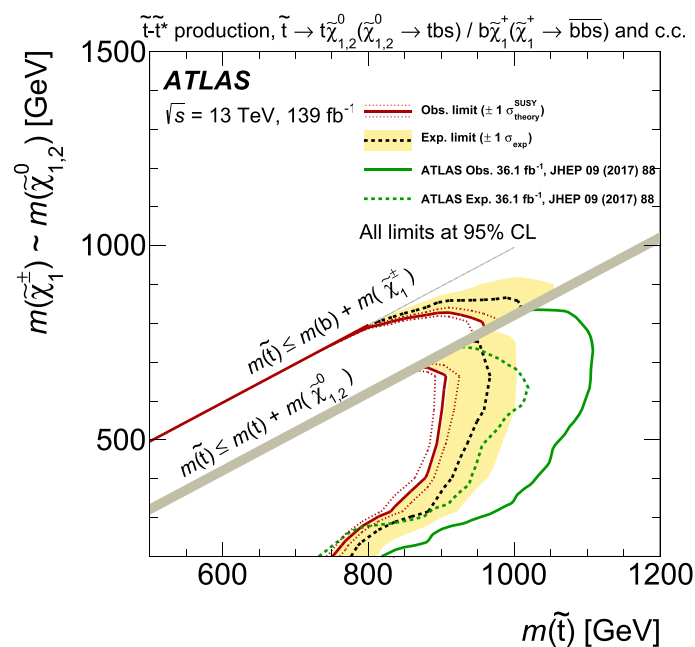
Fig. 8 Observed and expected exclusion contours for the \tilde{t} and \chi_1^\pm masses in a top-squark production model with RPV decays of the \chi_1^\pm and of the \chi_1^0 . Limits are shown in the case of a higgsino LSP. The contours of the band around the expected limit are the \pm 1\sigma variations, including all uncertainties except theoretical uncertainties in the signal cross-section. The dotted lines around the observed limit illustrate
