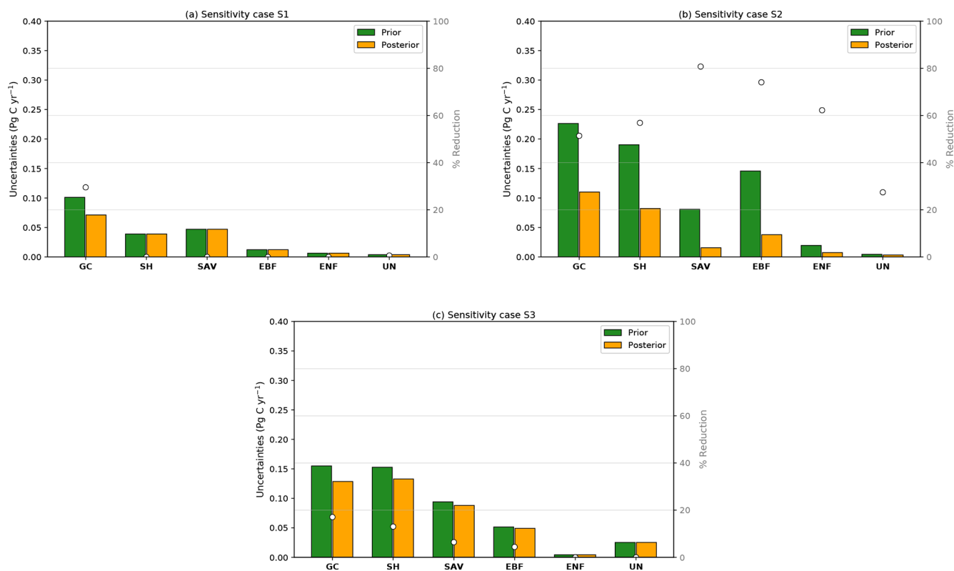
Figure 9. Sensitivity experiments for the prior and posterior uncertainties (in \text{Pg C yr}^{-1} ) aggregated over six different classes over the Australia domain using MODIS Land Cover Type Product (MCD12C1).
