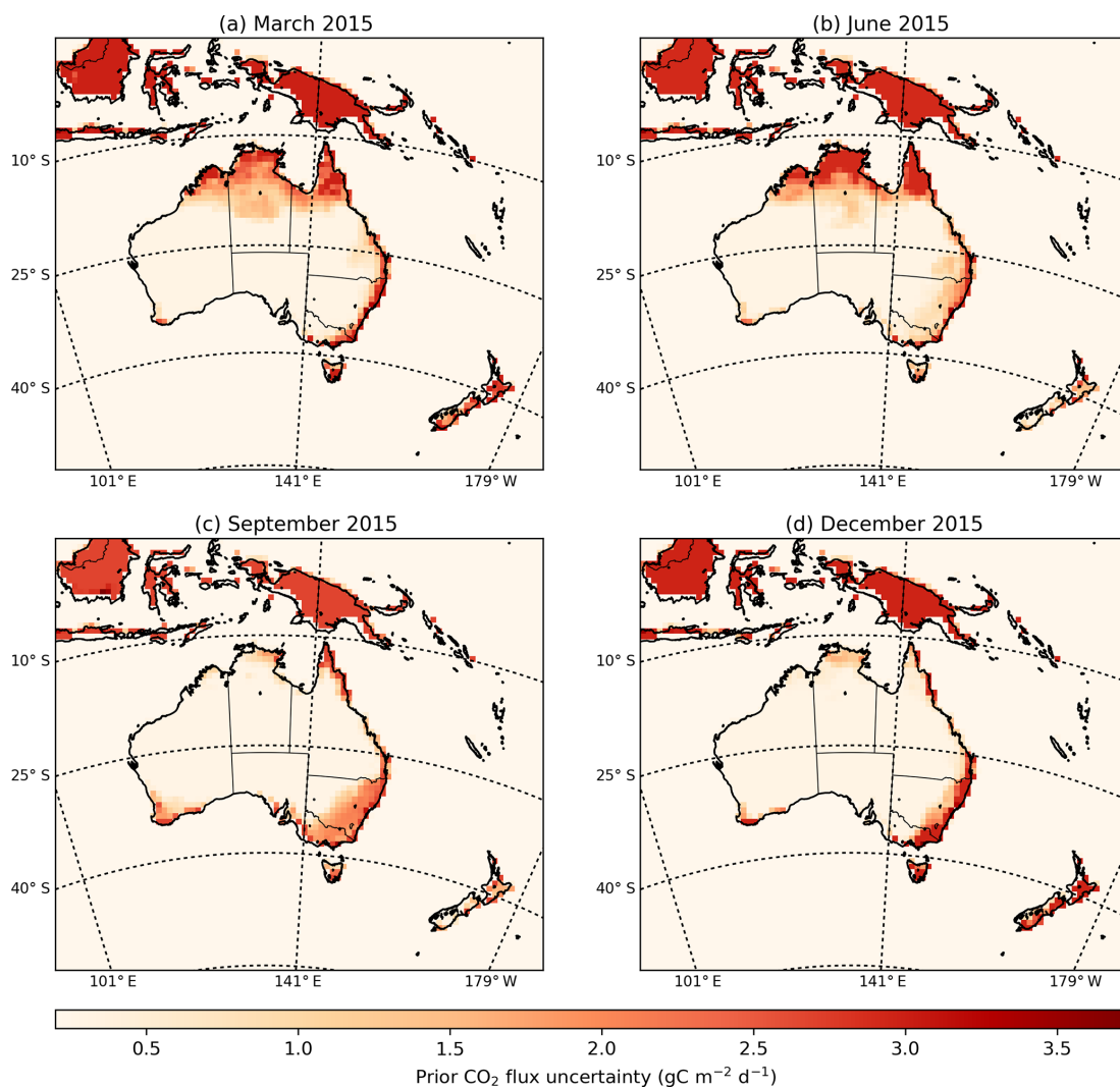
Figure 3. Monthly mean of CO 2 prior uncertainties accounting for the major terms in the CO 2 budget (anthropogenic fluxes, fires, land and ocean exchange) (in units of g C m -2 d -1 ).
