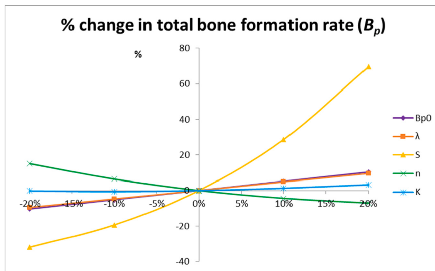
Fig. 8. Sensitivity analysis of the total bone formation rate ( B_p ) on depending parameters: basal bone formation rate ( B_{p0} ), new bone formation rate ( \lambda ), steepness of Hill's function ( n ), mechanical stimuli index ( S ) and activation coefficients ( K ).
