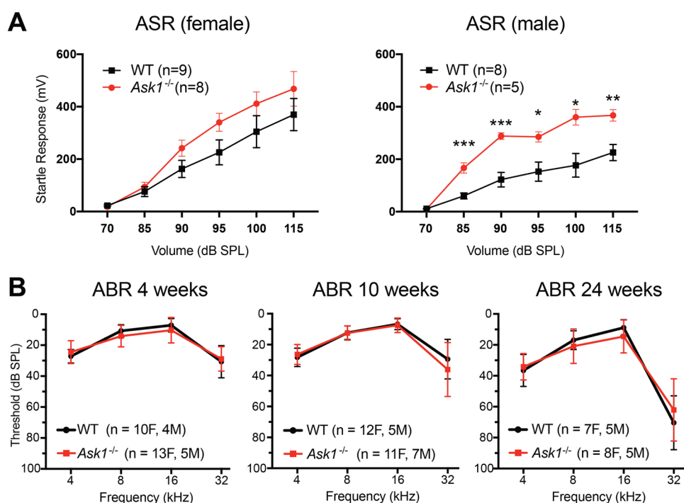
Fig. 2 The Ask1 -/- acoustic startle response and auditory brainstem response. A Ask1 -/- mice (red) tended to have a stronger acoustic startle response than wild type (WT) controls (black). This difference was statistically significant in the male cohort, as detected using multiple unpaired T tests, * indicates p < 0.05 , ** indicates p < 0.01 , *** indicates p < 0.001 . Error bars represent SEM. B The auditory brainstem response thresholds of Ask1 -/- (red) and WT (black) mice. There was no significant difference between the average hearing thresholds of Ask1 -/- and WT mice at 4, 10, and 24 weeks of age. Age-related, high-frequency hearing loss was evident in both Ask1 -/- and WT mice at 24 weeks of age. F=female, M=male, n =sample size. Error bars = S.D
