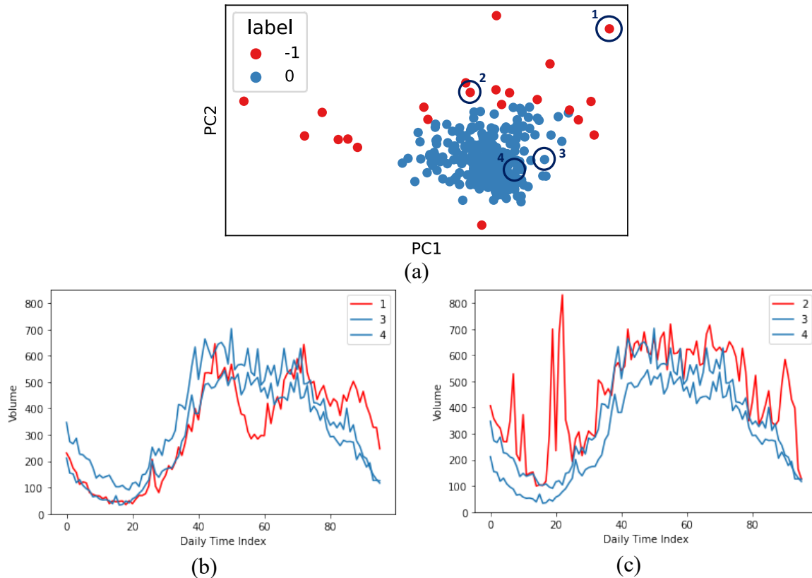
Figure 4: A close inspection of daily volume profiles mapped by the PCA into a 2-D space. Complete volume profiles related to the points spotted on (a) are demonstrated in (b) and (c). (Data derived from Hoddle St – Victoria St (S), Sunday)
