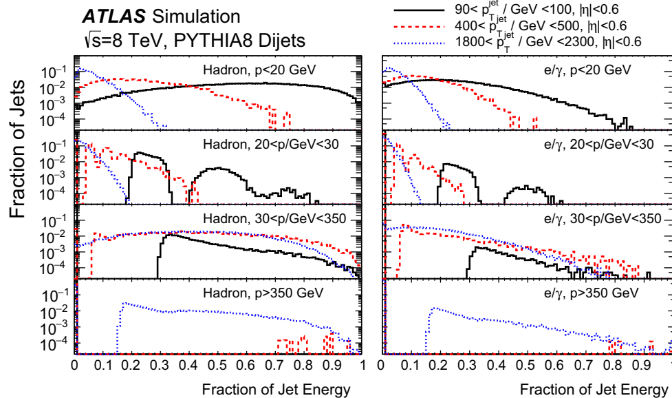
Fig. 34 The fraction of jet energy carried by particles in several categories (hadrons and EM particles, in several ranges of particle p ), for anti- k_t , R = 0.4 jets with 90 < p_T/\text{GeV} < 100 , 400 < p_T/\text{GeV} < 500 , or 1800 < p_T/\text{GeV} < 2300
