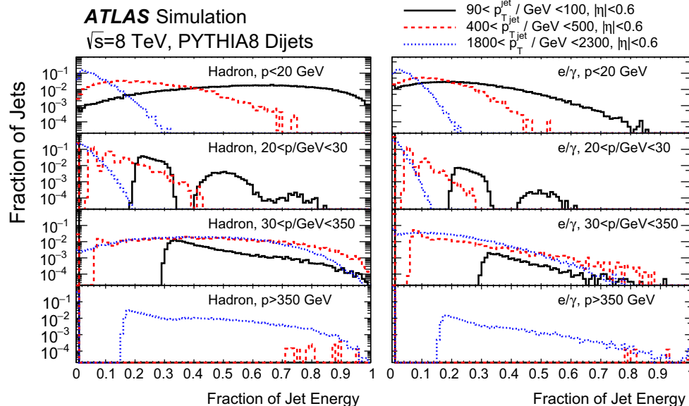
Fig. 34 The fraction of jet energy carried by particles in several categories (hadrons and EM particles, in several ranges of particle p ), for anti- k_t , R = 0.4 jets with 90 < p_T/\text{GeV} < 100 , 400 < p_T/\text{GeV} < 500 , or 1800 < p_T/\text{GeV} < 2300
