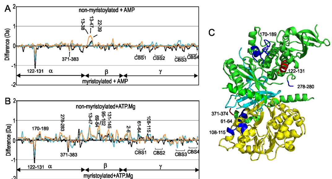
Figure 4. Comparison of deuterium uptake of myristoylated vs non-myristoylated AMPK bound to nucleotides. Difference of myristoylated and non-myristoylated AMPK bound to (A) AMP and (B) ATP.Mg 2+ . For each plot changes in deuteriation are shown at three time points: 1 min (orange), 5 min (blue) and 10 min (black). Each point is an average of two separate and independent experiments. On the y-axis a positive difference is indicative of increased deuteriation for peptides of the non-myristoylated AMPK titrated with ATP.Mg 2+ , whereas a negative difference is indicative of increased deuteriation for peptides of myristoylated AMPK titrated with ATP.Mg 2+ . On the x-axis are individual peptides; assignment of peptide to subunit is shown. (C) Location of peptides that show marked HDX differences in the \alpha - (green) and \gamma -subunits (yellow) for ATP.Mg 2+ are mapped onto the structure of AMPK (pdb 4CFH). The \alpha\gamma -SBS of the \beta -subunit is in cyan. Significant peptides that show faster HDX for myristoylated AMPK compared to non-myristoylated are mapped on the structure in red and those that show slower HDX for myristoylated AMPK compared to non-myristoylated are mapped on the structure in blue. The position of the \beta -CBM is unknown in this structure, however several peptides of the CBM show slow HDX for myristoylated AMPK.
