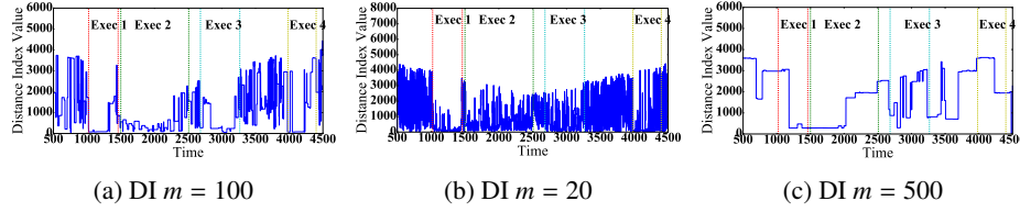
Fig. 4: Distance Index (DI) with various input parameter m for time series in Figure 1. In the repeating regions, DI stays flat at the value of the repeat period for the duration of the repeat period. Although susceptible, DI is more robust to changes in m .
