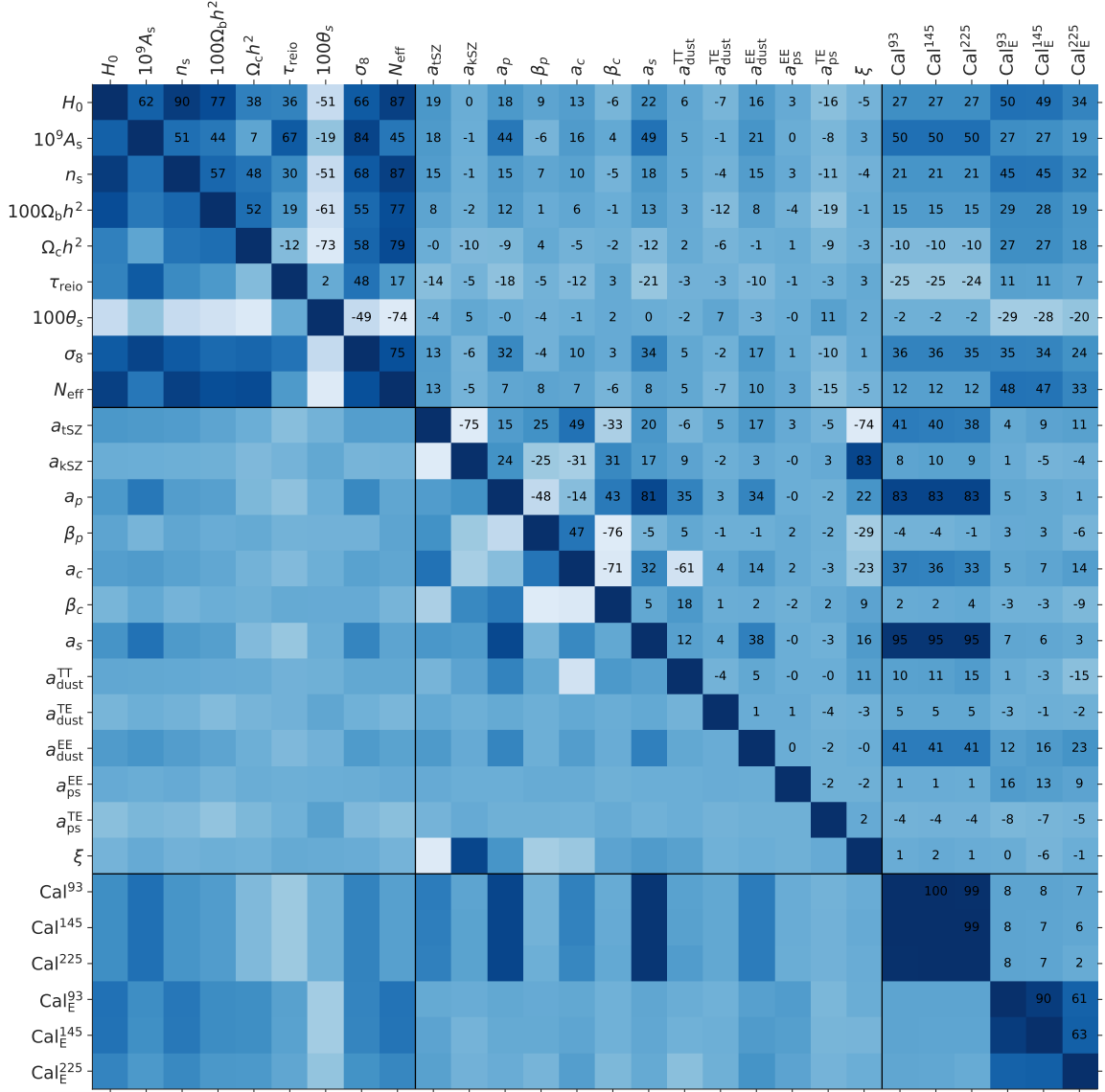
Figure 26. Correlation matrix for the case in which we marginalize over calibrations with Gaussian priors \mathcal{N}(1,0.01) GHz (label: \text{C}\mathcal{N}0.01\text{-smooth} ). The correlation factors are multiplied by 100.
